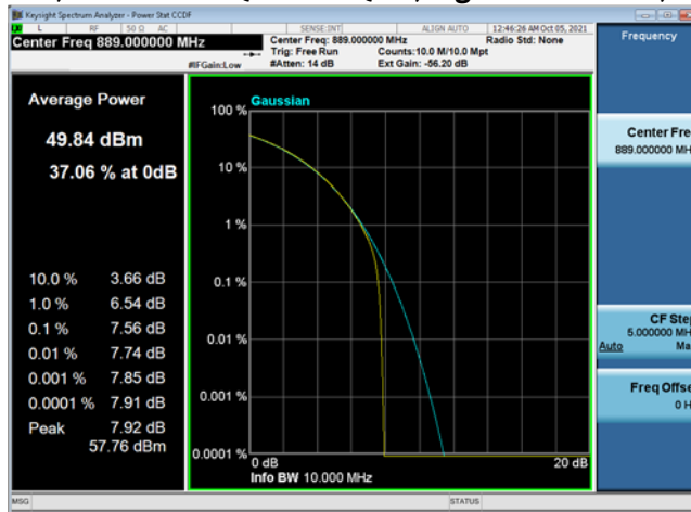
Test Model 3.2, Modulation QPSK/16QAM, Signal BW 10MHz, TX2, 889MHz
