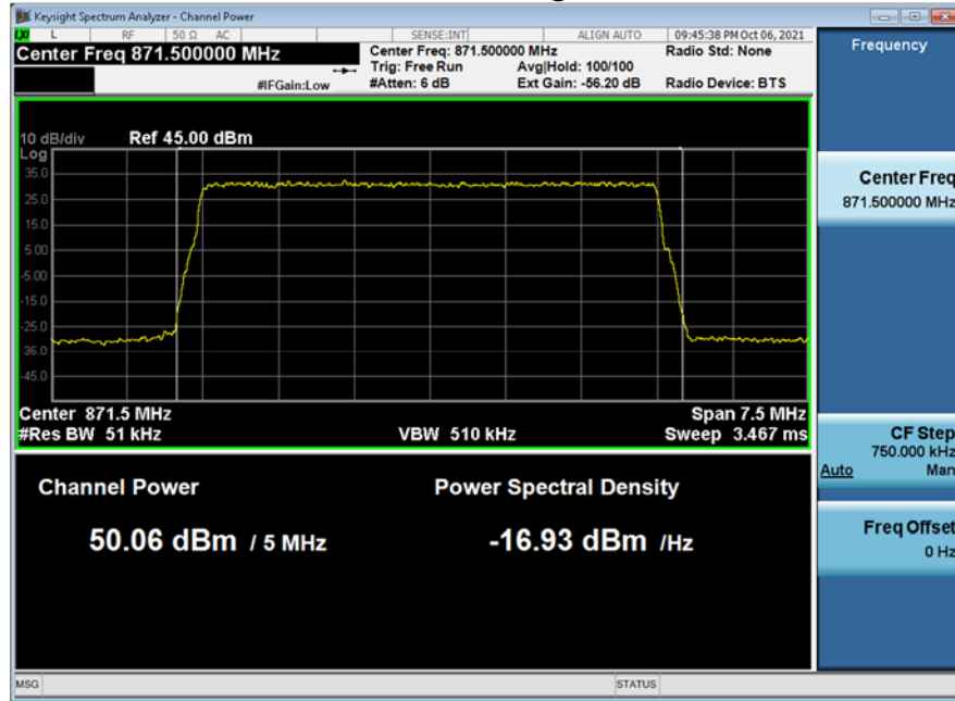
Test Model 3.1, Modulation 64QAM, Signal BW 5MHz, TX2, 871MHz
