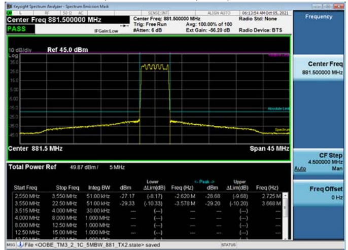
TM3.2, QPSK/16QAM, TX2, 881MHz
