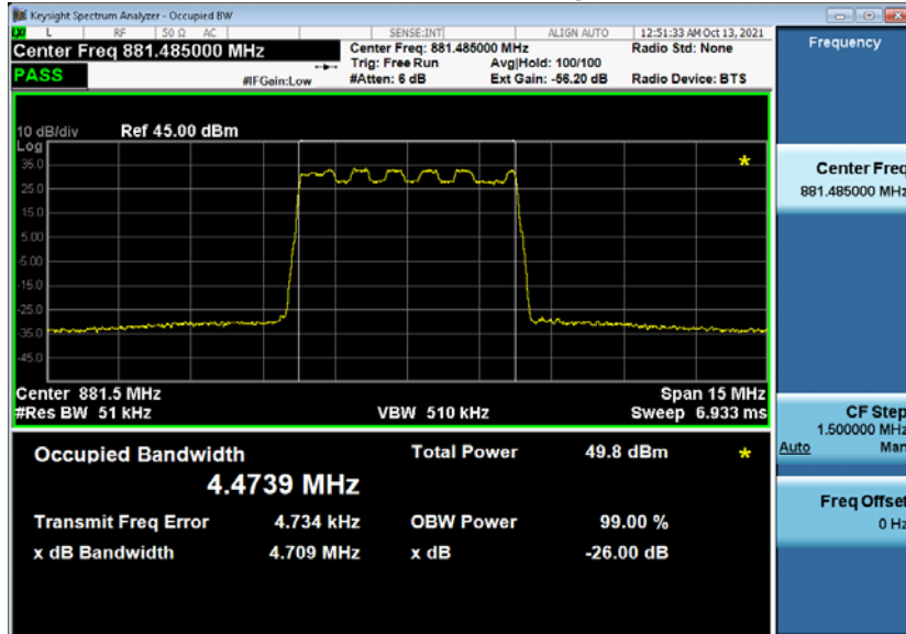
Test Model 3.2, Modulation QPSK/16QAM, Signal BW 5MHz, TX2, 881MHz
