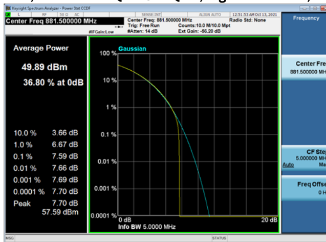
Test Model 3.2, Modulation QPSK/16QAM, Signal BW 5MHz, TX2, 881MHz
