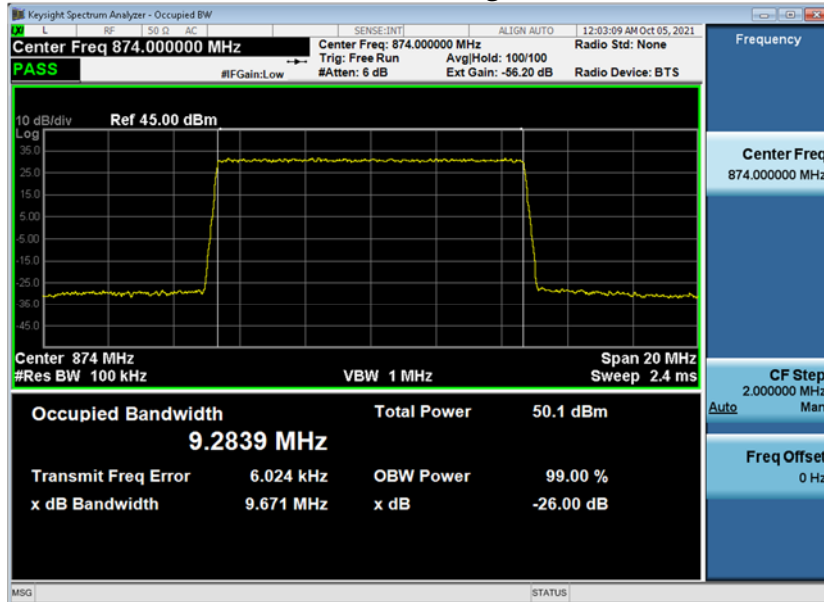
Test Model 3.1a, Modulation 256QAM, Signal BW 10MHz, TX2, 874MHz
