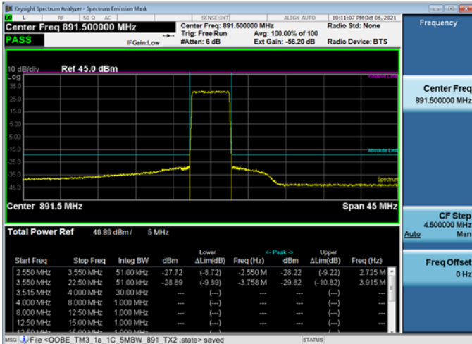
TM3.1a, 256QAM, TX2, 891MHz
