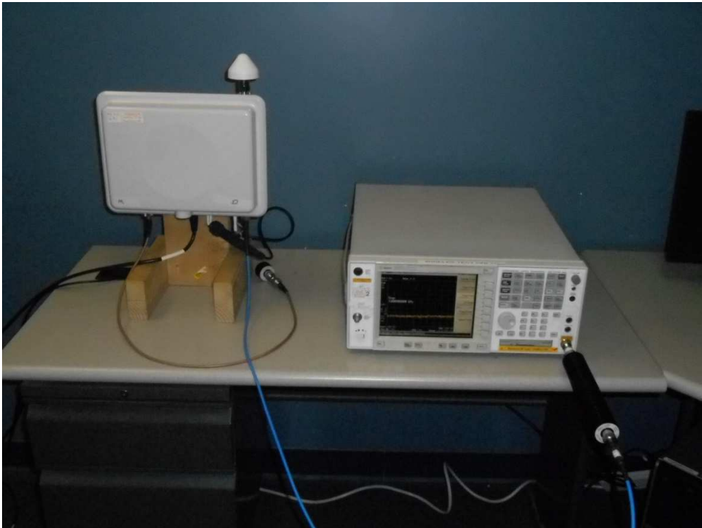
Antenna Port Conducted Tests
