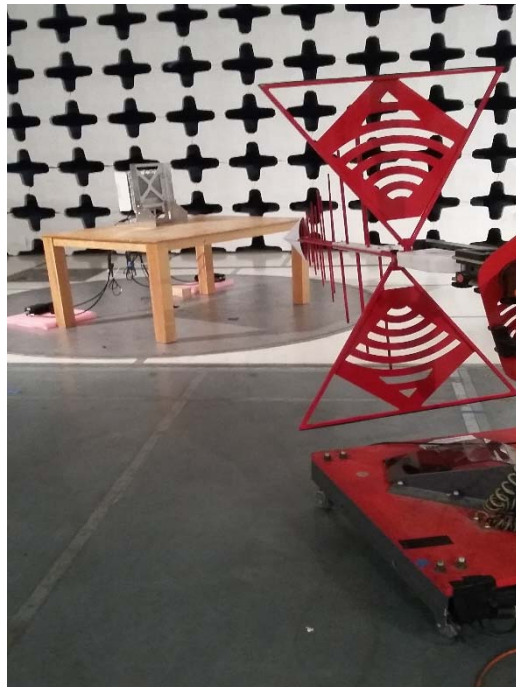
Radiated Spurious Emissions < 1GHz
