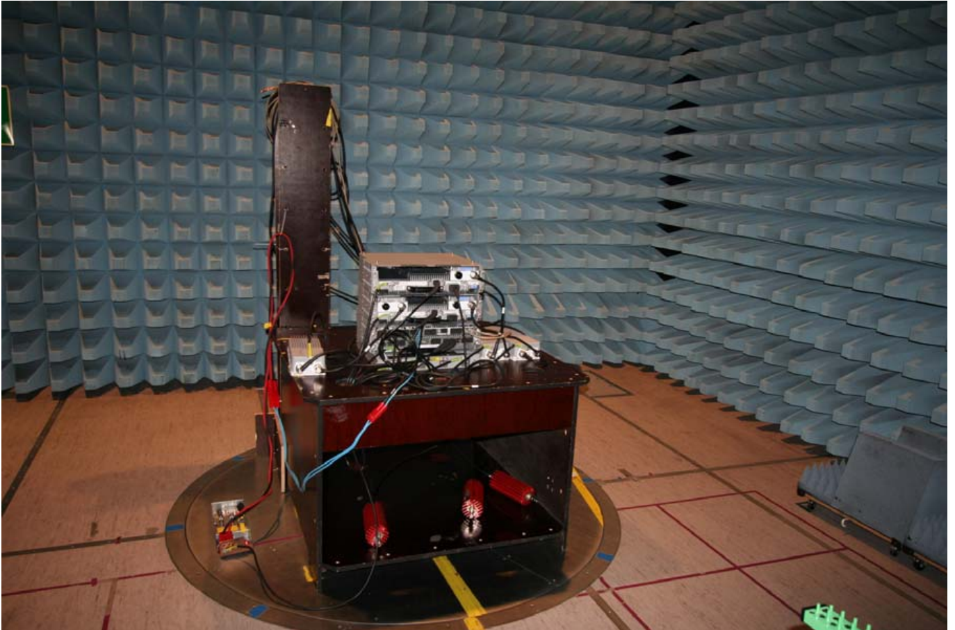
Photograph of Test Setup
