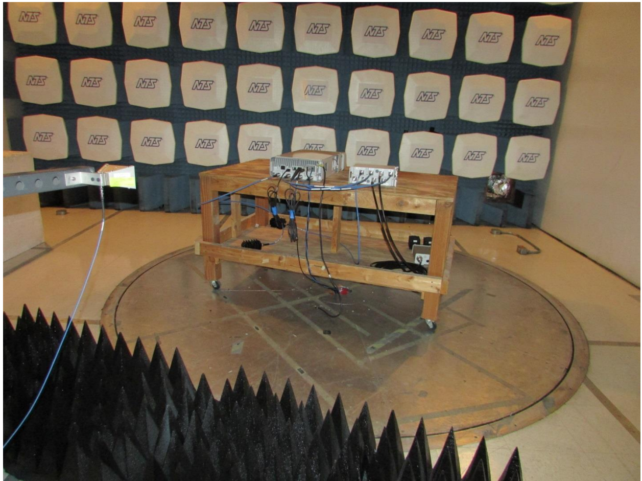
18-22GHz Radiated Measurements
