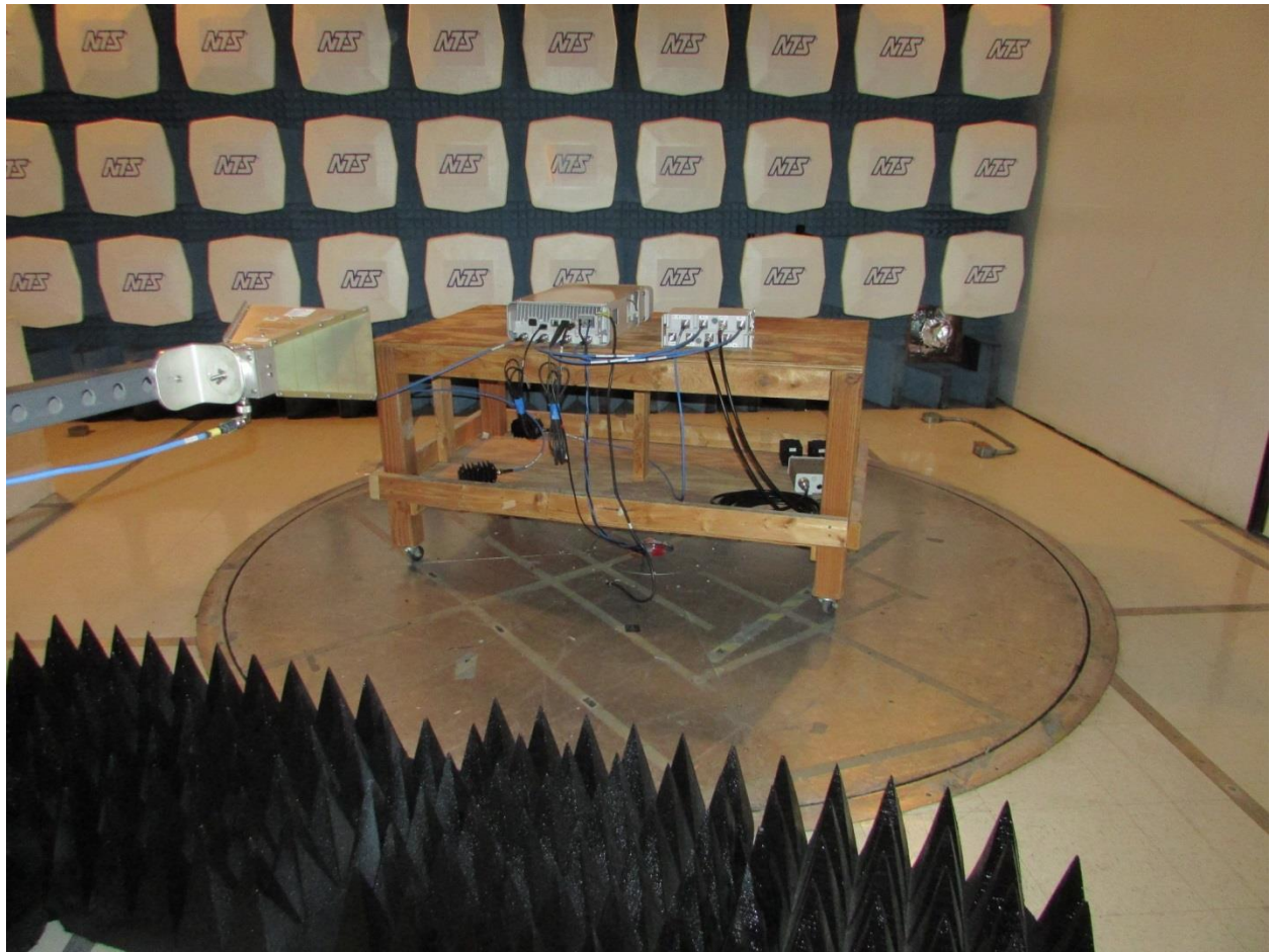
10-18GHz Radiated Measurements
