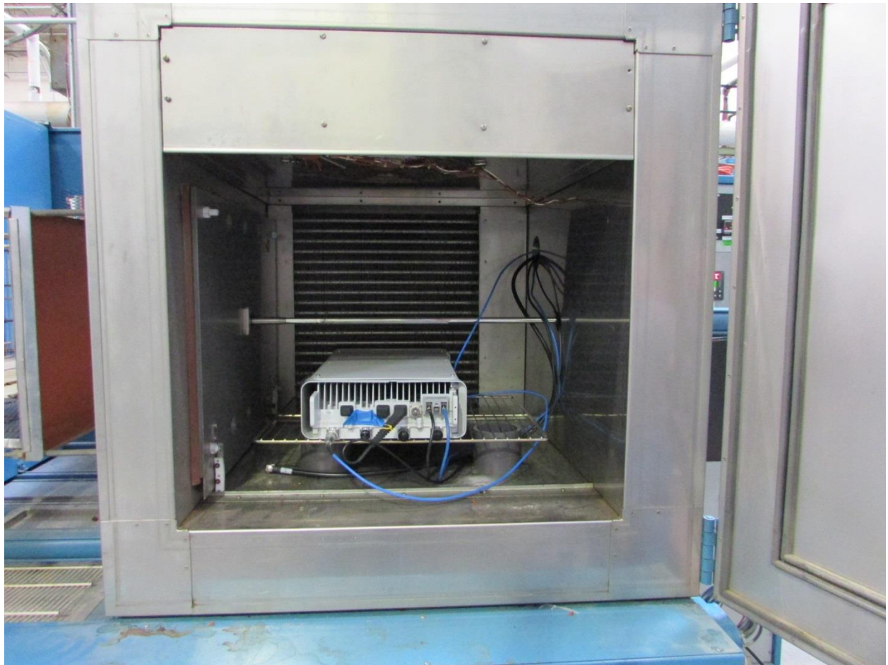
Frequency Stability measurement
