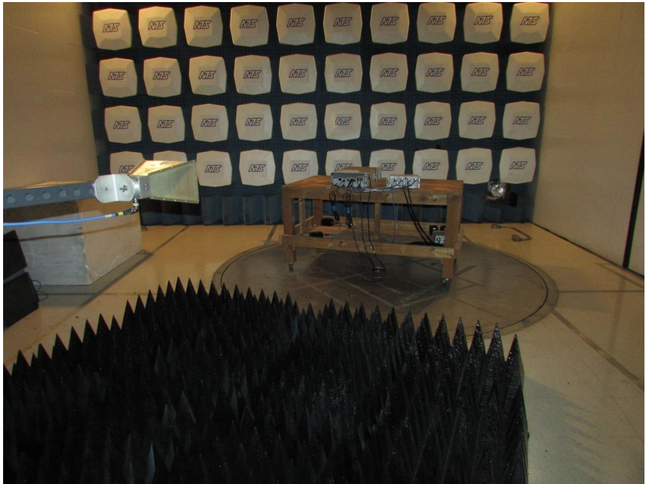
1-10GHz Radiated Measurements
