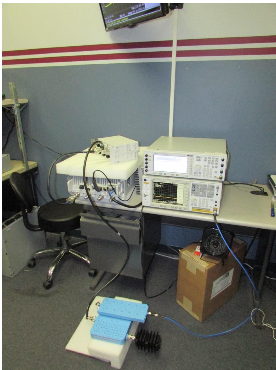
AWS - 4 Band Out of Band Emissions test setup
