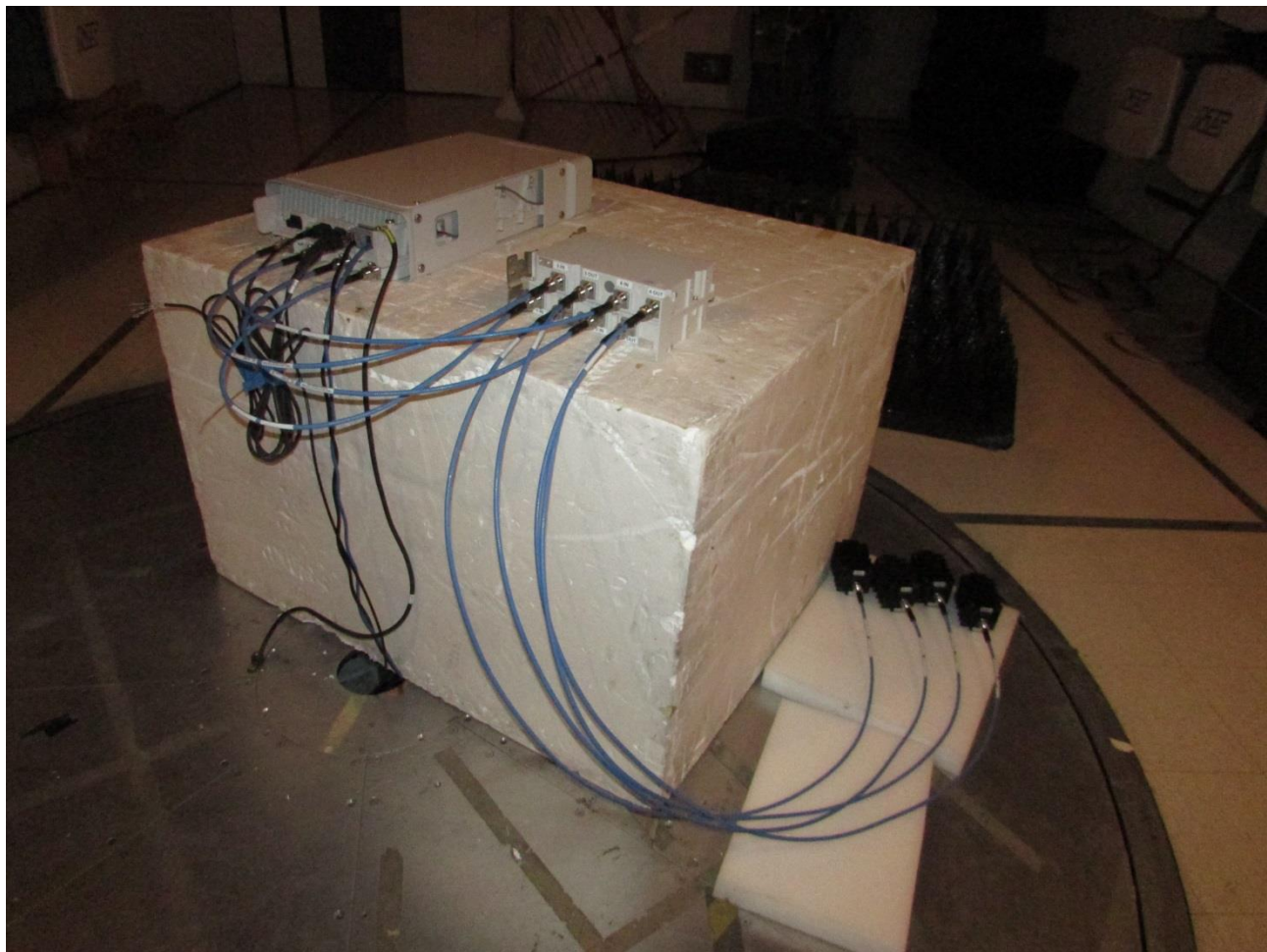
AWS - 4 Band Out of Band Radiated Emissions test setup (Back)
