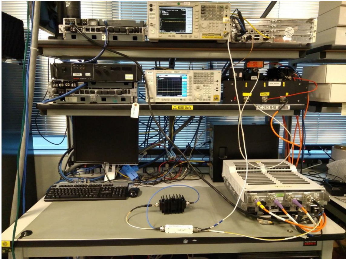
FRIG NB-IoT GB test setup below 10 MHz
