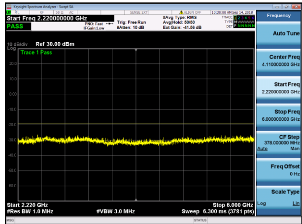
LTE20 BOTTOM+NB IoT GB (Upper) 2220MHz-6000MHz
