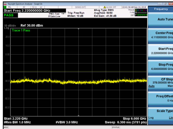
LTE20 Mid+NB IoT GB (Upper) 2220MHz-6000MHz
