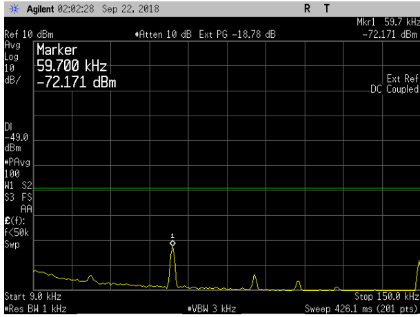
LTE15 Mid+NB IoT GB (Upper) 0.009-0.15MHz
