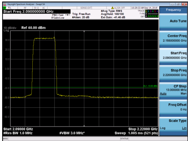
LTE20 BOTTOM+NB IoT GB (Upper) 2090MHz – 2220MHz
