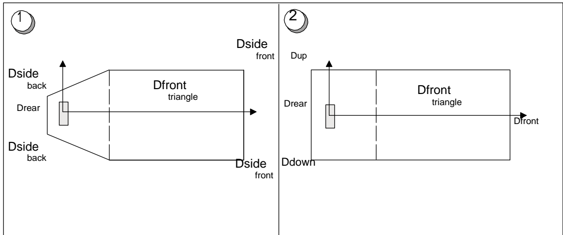
Figure 4 Antenna side and top view
