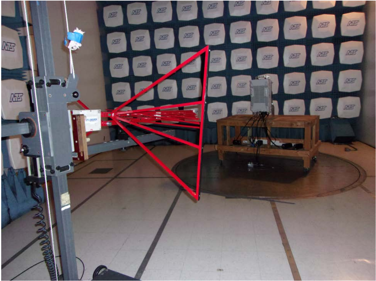
Radiated Spurious Emissions 30-1000MHz
