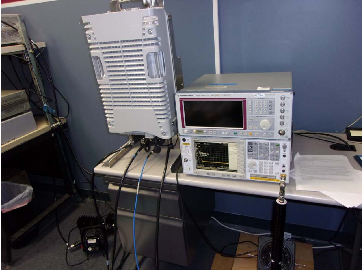
General Conducted Port Measurements
