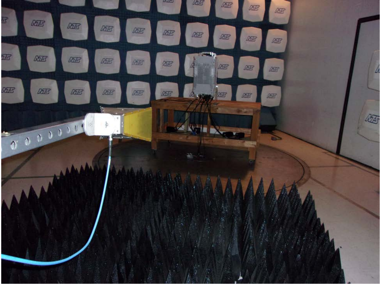
Radiated Spurious Emissions 1-10GHz
