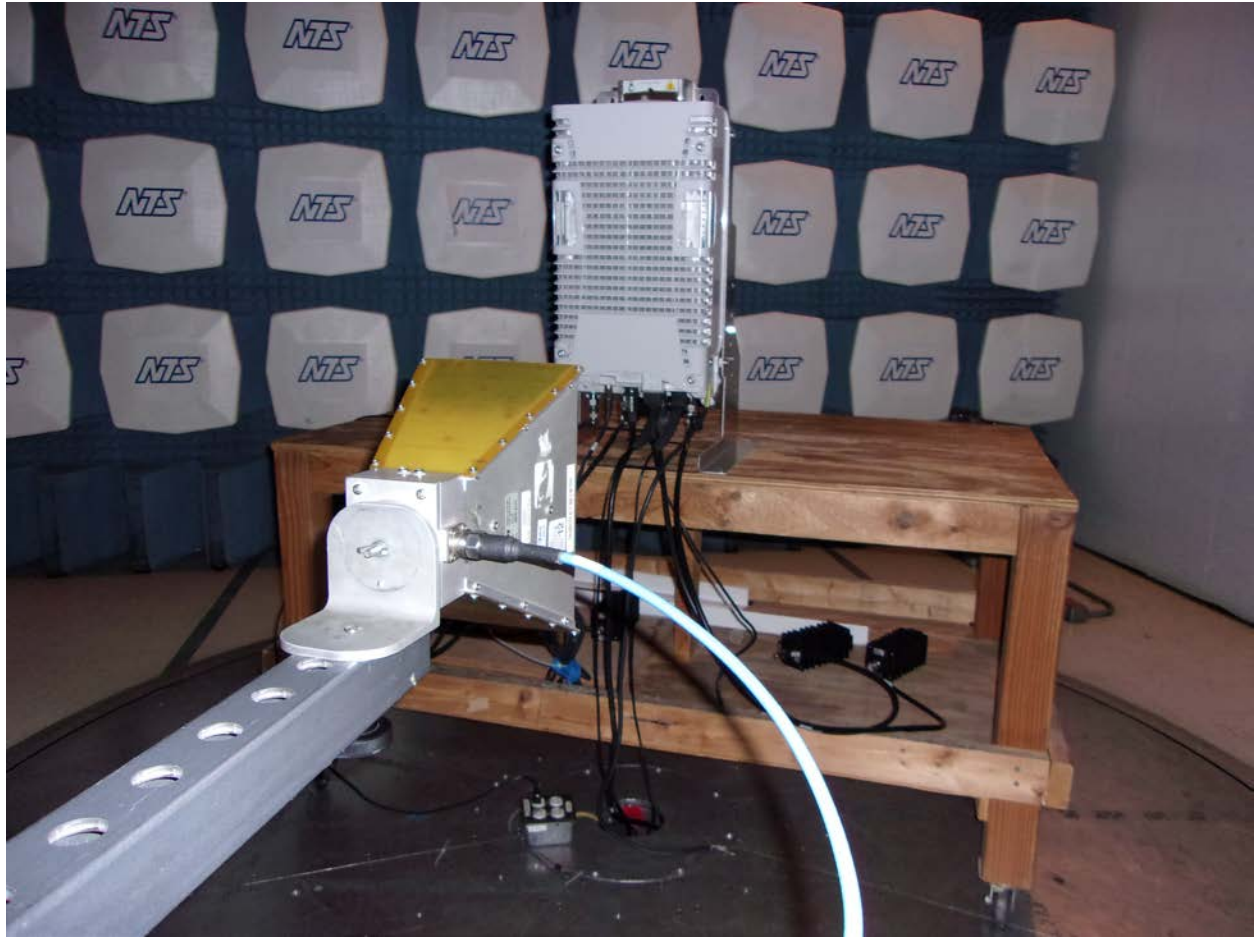
Radiated Spurious Emissions 10-13GHz
