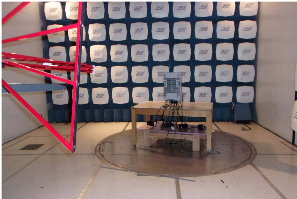
Radiated Spurious Emissions 30-1000MHz
