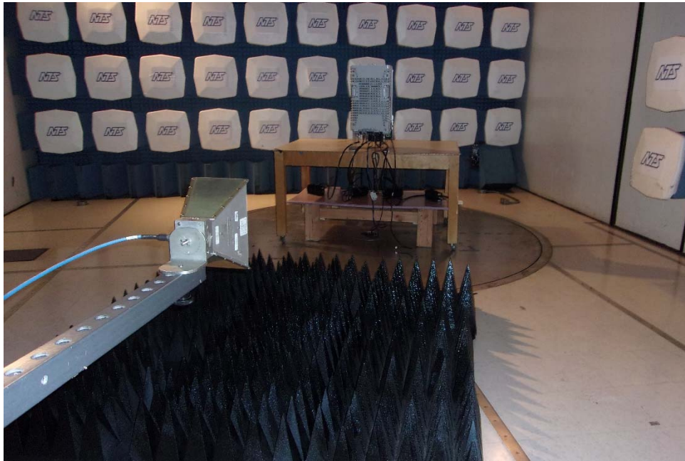
Radiated Spurious Emissions 1-7GHz
