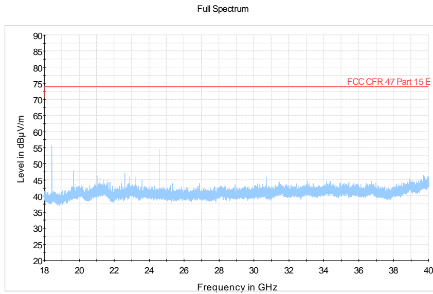
Figure 407 Radiated Emission 18GHz – 40 GHz (5745MHz) (20MHz Channel BW)
