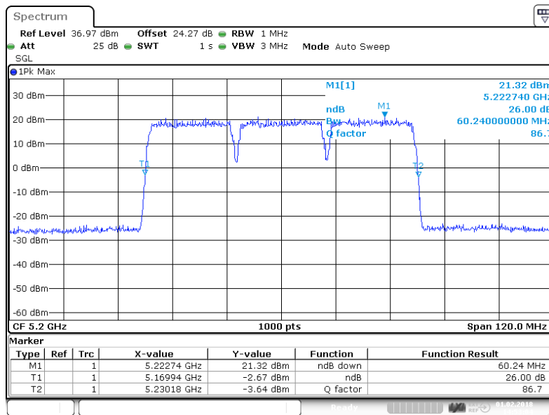
Figure 83 Occupied Bandwidth – 16QAM (5180/ 5200/5220 MHz) (2 X 20MHz Channel BW)
