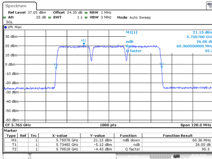
Figure 86 Occupied Bandwidth – 64QAM (5745.0/ 5765.0/ 5785.0 MHz) (20MHz Channel BW)
