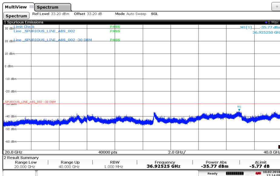
Figure 181 Spurious Emissions (20 GHz – 40 GHz) – 64QAM (5785.0 MHz) (20MHz Channel BW)
