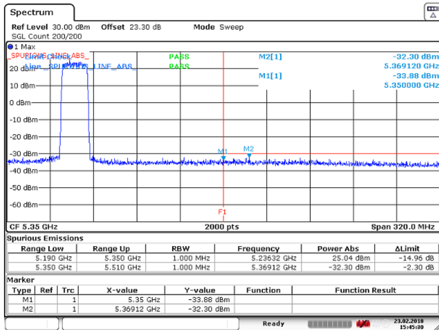
Figure 9 Spurious Emissions (Upper Band Edge) – 16QAM (5240.0 MHz) (20MHz Channel BW)
