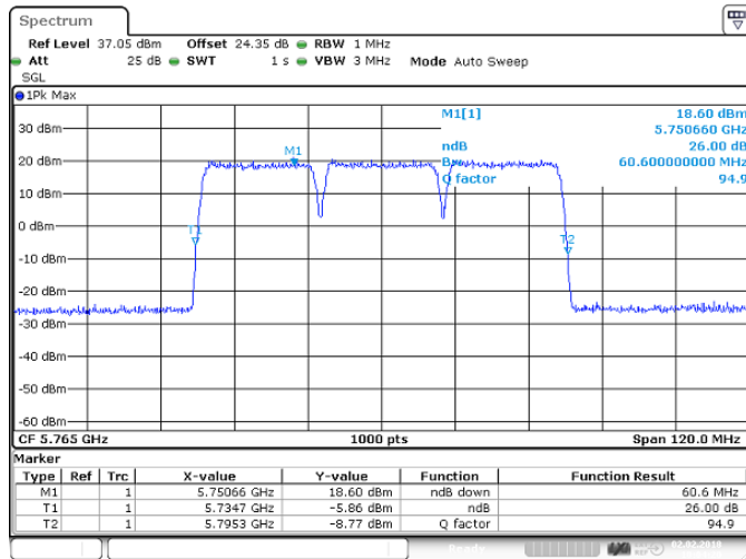
Figure 85 Occupied Bandwidth – QPSKQAM (5745.0/ 5765.0/ 5785.0 MHz) (20MHz Channel BW)
