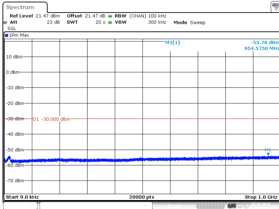
Figure 168 Spurious Emissions (9 kHz – 1 GHz) – QPSK (5785.0 MHz) (20MHz Channel BW)
