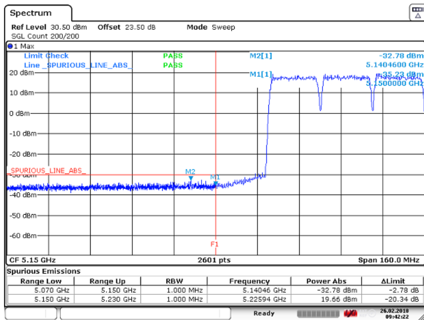
Figure 136 Spurious Emissions (Lower Band Edge) – QPSK (5180.0/ 5200.0/ 5220 MHz) (3 X 20MHz Channel BW)
