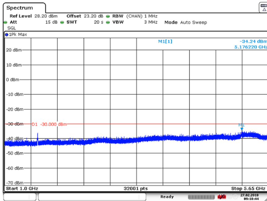
Figure 172 Spurious Emissions (1 GHz – 5.65 GHz) – QPSK (5785.0 MHz) (20MHz Channel BW)
