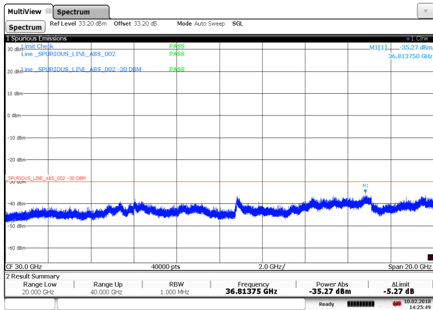
Figure 135 Spurious Emissions (20 GHz – 40 GHz) – 256QAM (5200.0/ 5220.0 MHz) (2 X 20MHz Channel BW)
