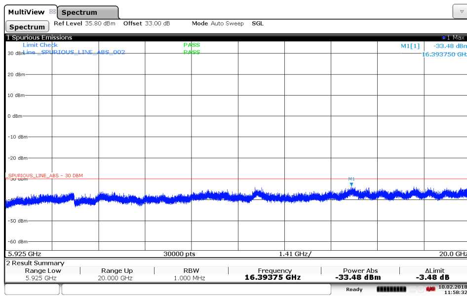
Figure 176 Spurious Emissions (5.925 GHz – 20 GHz) – QPSK (5785.0 MHz) (20MHz Channel BW)
