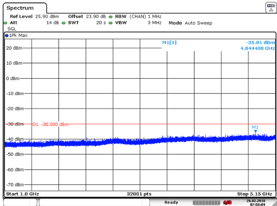
Figure 102 Spurious Emissions (1 GHz – 5.15 GHz) – 16QAM (5220.0 MHz) (20MHz Channel BW)
