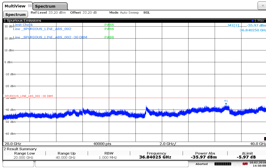
Figure 156 Spurious Emissions (20 GHz – 40 GHz) – QPSK (5200.0/ 5200/ 5220 MHz) (3 X 20MHz Channel BW)
