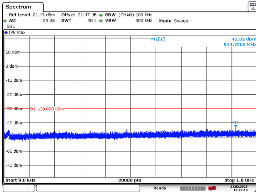
Figure 122 Spurious Emissions (9 kHz – 1 GHz) – 16QAM (5200.0/ 5220.0 MHz) (2 X 20MHz Channel BW)
