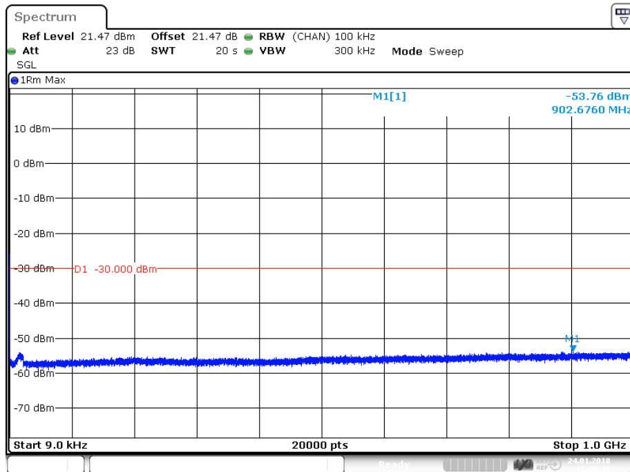
Figure 96 Spurious Emissions (9 kHz – 1 GHz) - QPSK (5220.0 MHz) (20MHz Channel BW)
