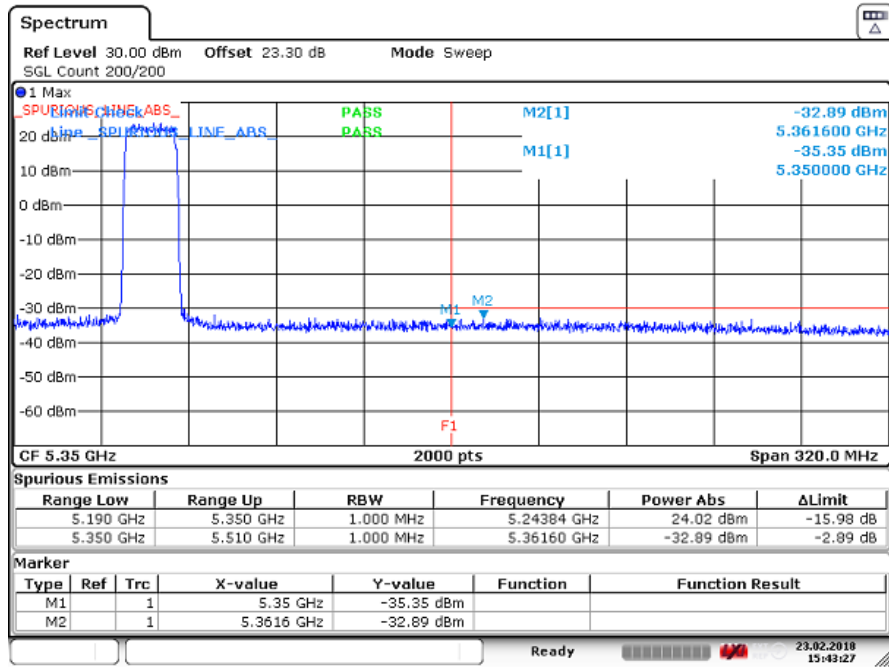
Figure 9 Spurious Emissions (Upper Band Edge) – 64QAM (5240.0 MHz) (20MHz Channel BW)
