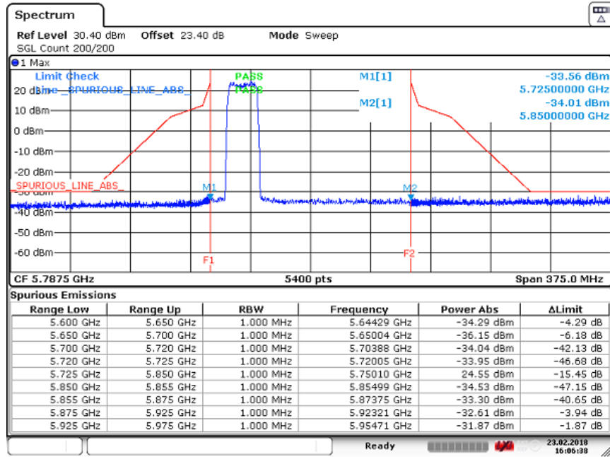
Figure 160 Spurious Emissions (Lower Band Edge) – QPSK (5745.0 MHz) (20MHz Channel BW)
