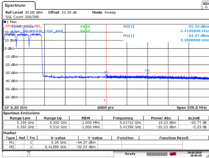
Figure 143 Spurious Emissions (Upper Band Edge) – 256QAM (5200.0/ 5220.0/ 5240 MHz) (3 X 20MHz Channel BW)
