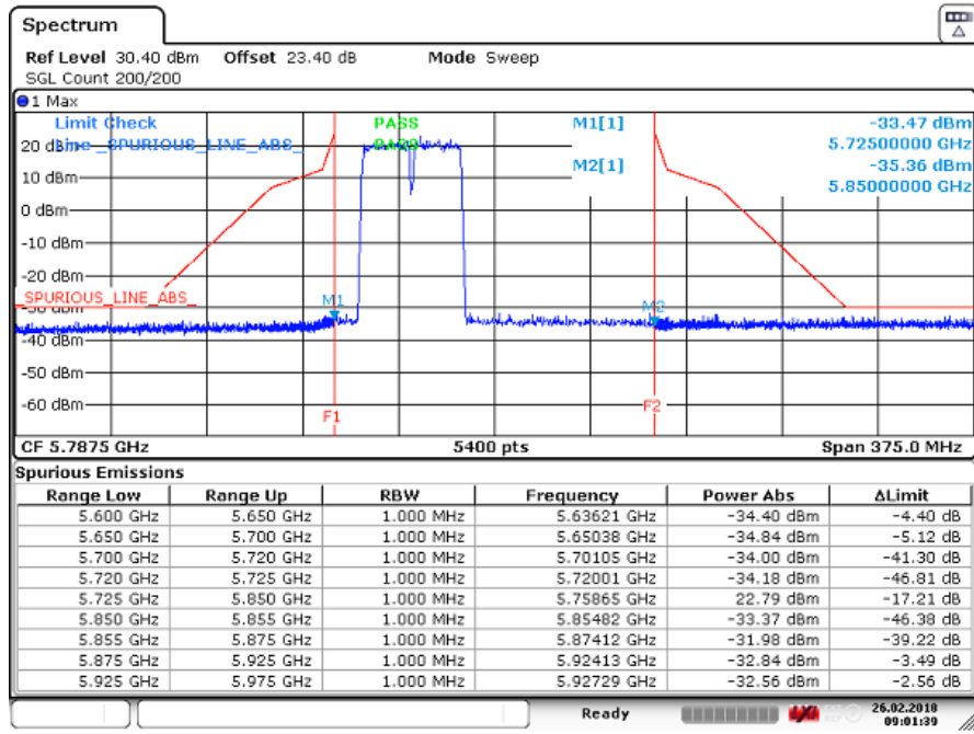
Figure 186 Spurious Emissions (Lower Band Edge) – 16QAM (5745.0/ 5765.0 MHz) (2 X 20MHz Channel BW)
