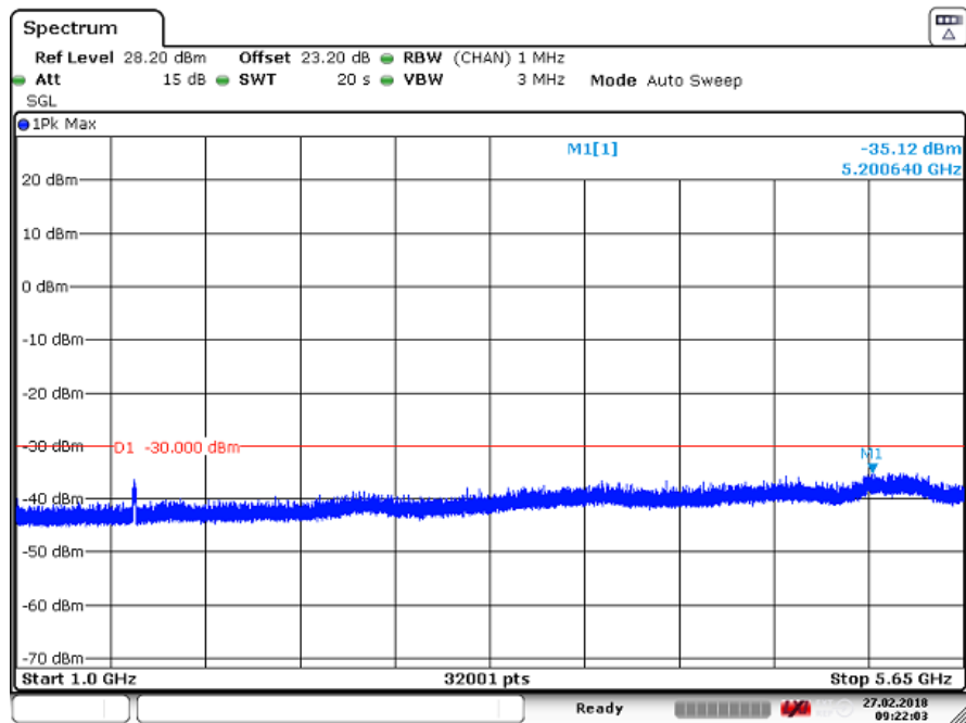
Figure 174 Spurious Emissions (1 GHz – 5.65 GHz) – 16QAM (5785.0 MHz) (20MHz Channel BW)
