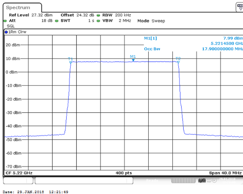
Figure 30 Occupied Bandwidth – 64QAM (5220.0 MHz) (20MHz Channel BW)
