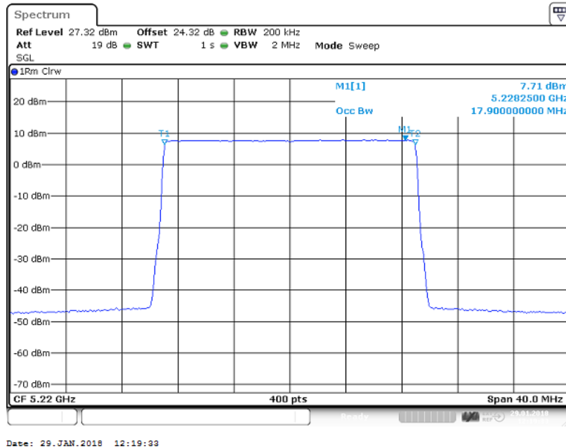
Figure 29 Occupied Bandwidth – QPSK (5220.0 MHz) (20MHz Channel BW)
