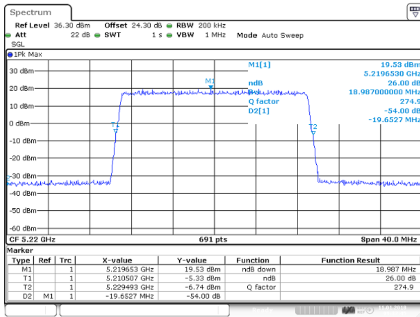
Figure 38 Occupied Bandwidth – 64QAM (5220.0 MHz) (20MHz Channel BW)
