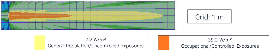
Figure 14 – Side view of the power density for the time-averaged maximum transmitted power of 339 W and the beam oriented in azimuth = 0° & elevation = 0° (Canada)
