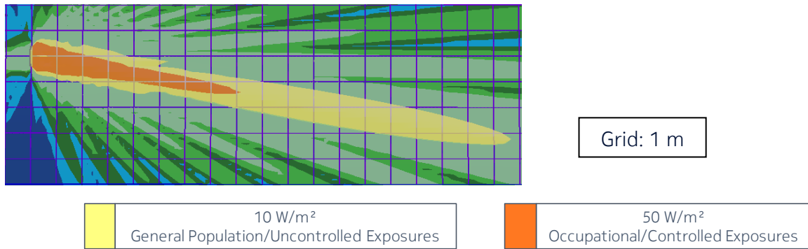
Figure 4 – Side view of the power density for the time-averaged maximum transmitted power of 339 W and the beam oriented in azimuth = 0° & elevation = +10° (EU/ICNIRP, Australia/NZ and US/related)
