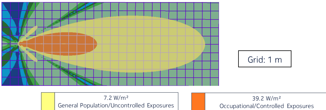
Figure 10 – Top view of the power density for the time-averaged maximum transmitted power of 339 W and the beam oriented in azimuth = 0° & elevation = 0° (Canada)
