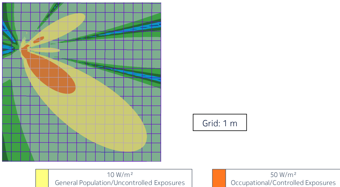
Figure 8 – Top view of the power density for the time-averaged maximum transmitted power of 339 W and the beam oriented in azimuth = -40° & elevation = 0° (EU/ICNIRP, Australia/NZ and US/related)
