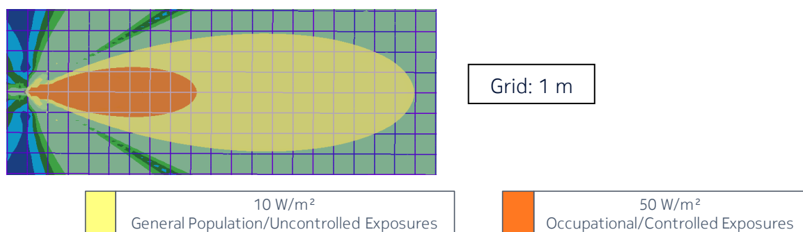
Figure 2 – Top view of the power density for the time-averaged maximum transmitted power of 339 W and the beam oriented in azimuth = 0° & elevation = 0° (EU/ICNIRP, Australia/NZ and US/related)
