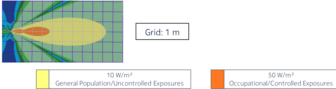
Figure 3 – Top view of the power density for the time-averaged actual maximum transmitted power of 85 W and the beam oriented in azimuth = 0° & elevation = 0° (EU/ICNIRP, Australia/NZ and US/related)
