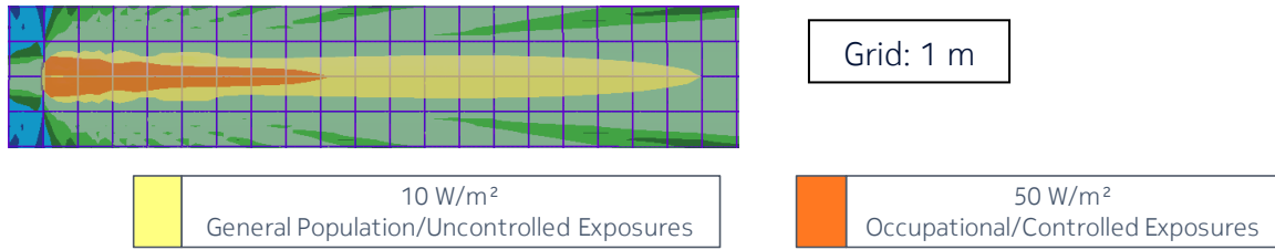
Figure 6 – Side view of the power density for the time-averaged maximum transmitted power of 339 W and the beam oriented in azimuth = 0° & elevation = 0° (EU/ICNIRP, Australia/NZ and US/related)
