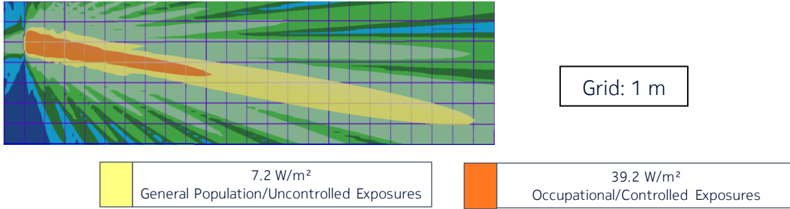
Figure 12 – Side view of the power density for the time-averaged maximum transmitted power of 339 W and the beam oriented in azimuth = 0° & elevation = +10° (Canada)
