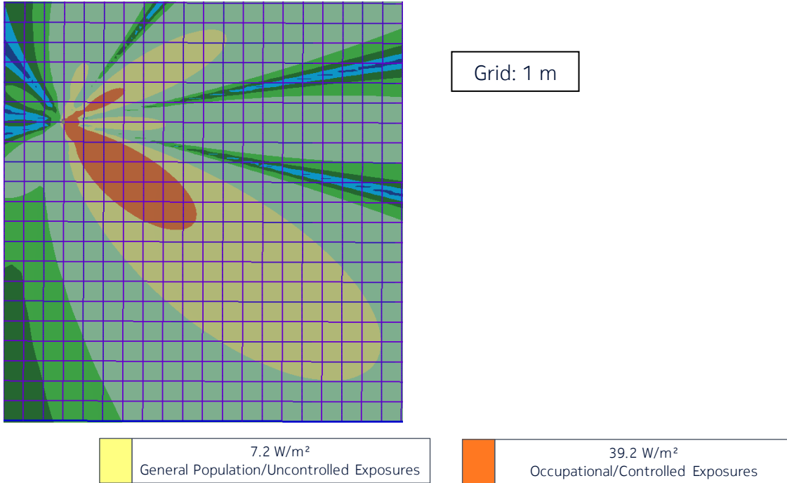
Figure 16 – Top view of the power density for the time-averaged maximum transmitted power of 339 W and the beam oriented in azimuth = -40° & elevation = 0° (Canada)
