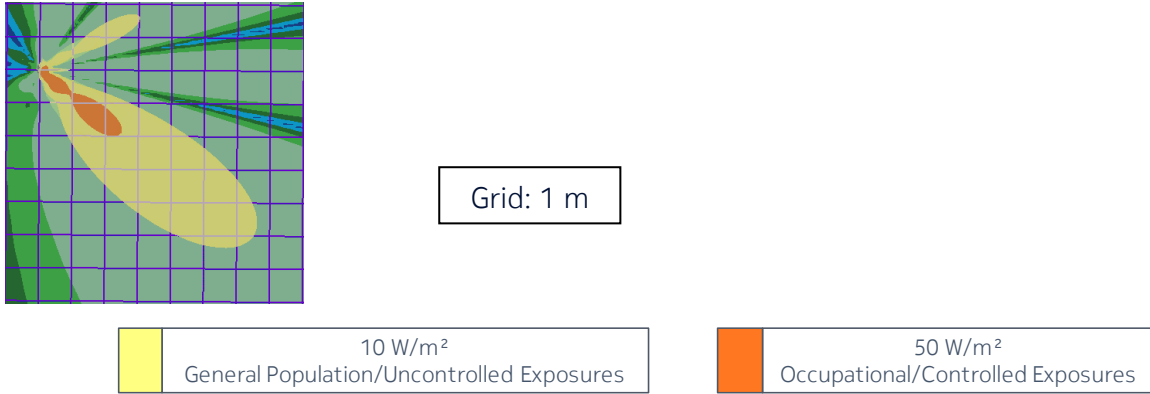
Figure 9 – Top view of the power density for the time-averaged actual maximum transmitted power of 85 W and the beam oriented in azimuth = -40° & elevation = 0° (EU/ICNIRP, Australia/NZ and US/related)
