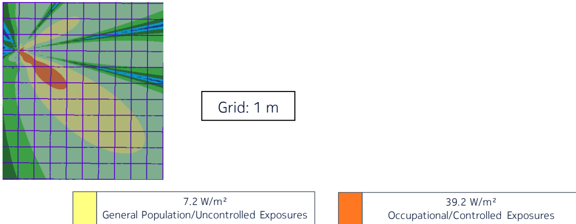
Figure 17 – Top view of the power density for the time-averaged actual maximum transmitted power of 85 W and the beam oriented in azimuth = -40° & elevation = 0° (Canada)
