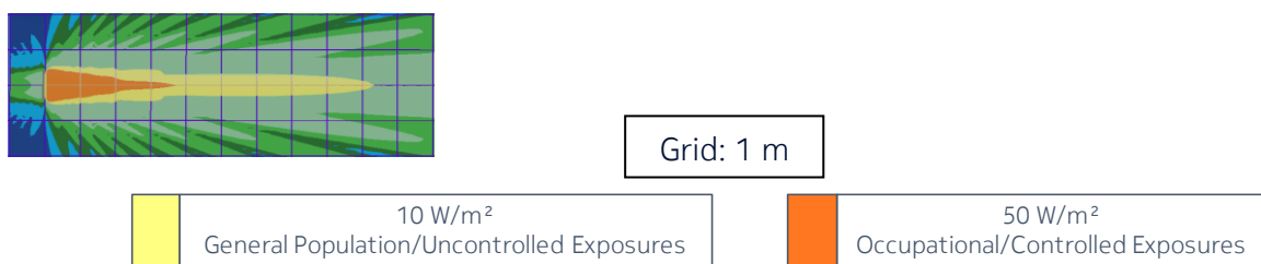
Figure 7 – Side view of the power density for the time-averaged actual maximum transmitted power of 85 W and the beam oriented in azimuth = 0° & elevation = 0° (EU/ICNIRP, Australia/NZ and US/related)
