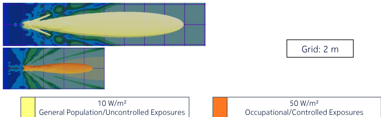
Figure 3 - Top view of the power density for the actual maximum transmitted power of 106 W (corresponding to the actual EIRP threshold of 75.1 dBm) and beam oriented in azimuth = 0° & elevation = +6° with a gain of 24.8 dBi (EU/ICNIRP, Australia/NZ and US/related)
