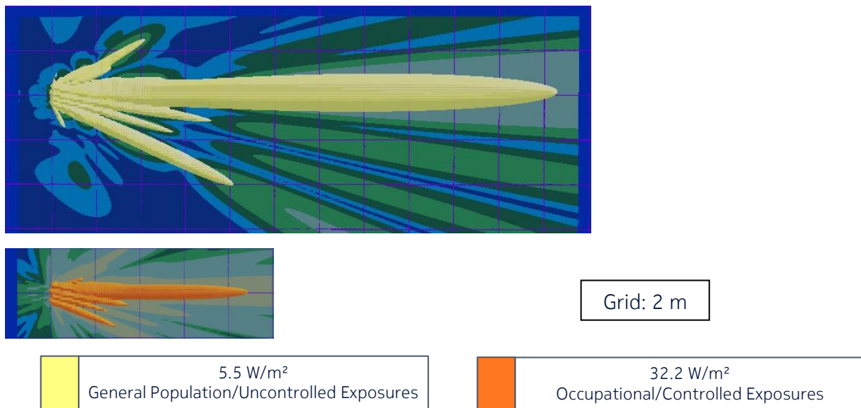
Figure 17 – Side view of the power density for the actual maximum transmitted power of 137 W (corresponding to the actual EIRP threshold of 75.1 dBm) and beam oriented in azimuth = -5° & elevation = -1° with a gain of 23.7 dBi (Canada)
