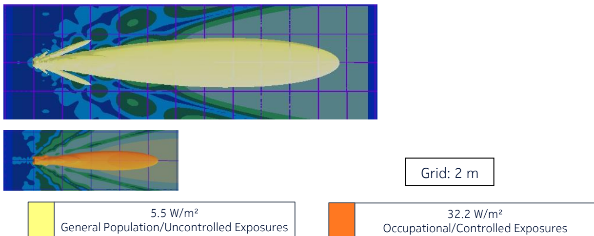
Figure 11 – Top view of the power density for the actual maximum transmitted power of 106 W (corresponding to the actual EIRP threshold of 75.1) and beam oriented in azimuth = 0° & elevation = +6° with a gain of 24.8 dBi (Canada)
