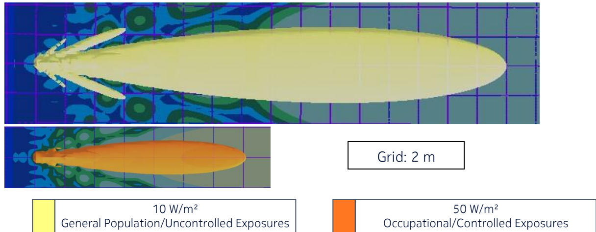
Figure 2 – Top view of the power density for the time-averaged maximum transmitted power of 424 W and beams oriented in azimuth = 0° & elevation = +6° with a gain of 24.8 dBi (EU/ICNIRP, Australia/NZ and US/related)
