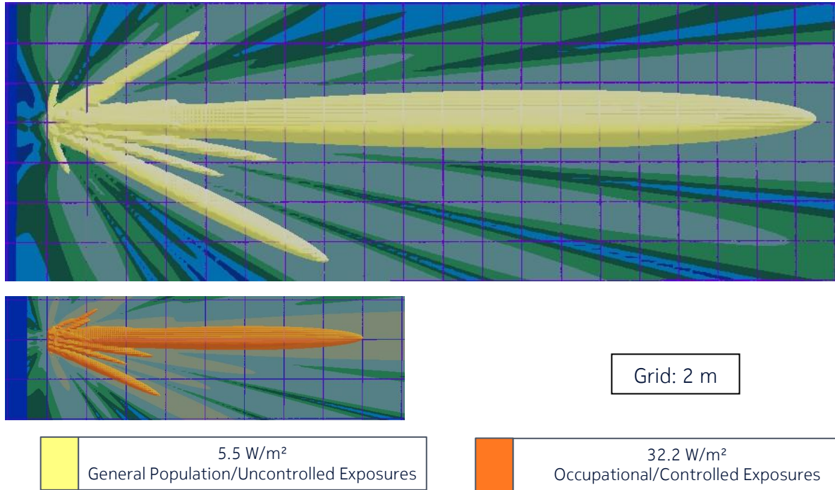
Figure 16 – Side view of the power density for the time-averaged maximum transmitted power of 424 W and beam oriented in azimuth = -5° & elevation = -1° with a gain of 23.7 dBi (Canada)
