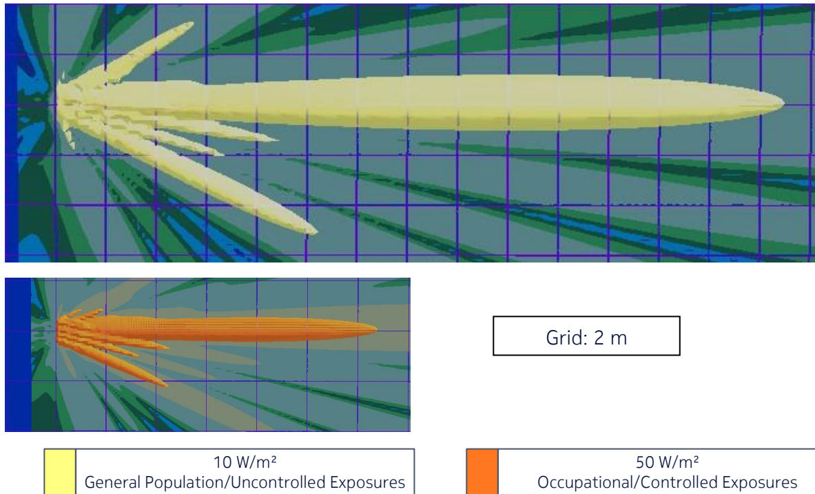
Figure 8 – Side view of the power density for the time-averaged maximum transmitted power of 424 W and beam oriented in azimuth = -5° & elevation = -1° with a gain of 23.7 dBi (EU/ICNIRP, Australia/NZ and US/related)
