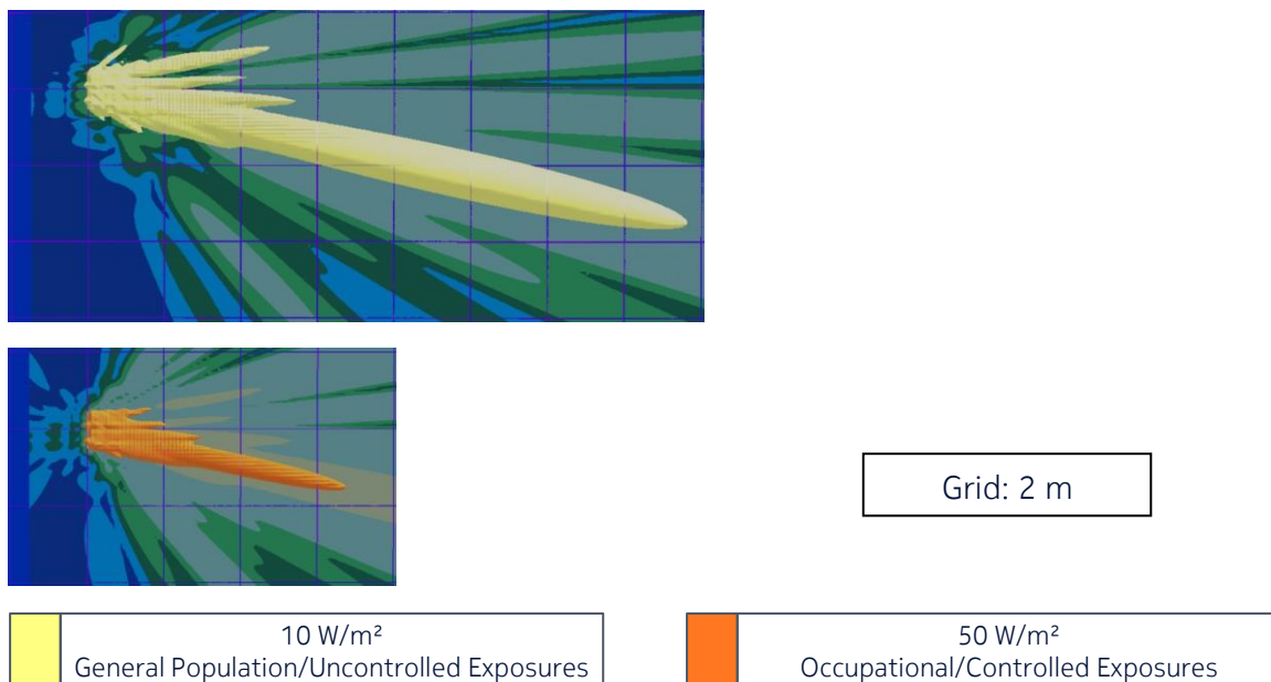
Figure 7 – Side view of the power density for the actual maximum transmitted power of 128 W (corresponding to the actual EIRP threshold of 75.1 dBm) and beam oriented in azimuth = +3° & elevation = +13° with a gain of 24.0 dBi (EU/ICNIRP, Australia/NZ and US/related)
