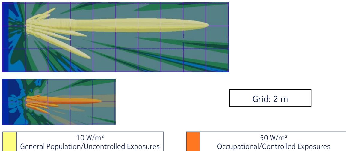
Figure 9 - Side view of the power density for the actual maximum transmitted power of 137 W (corresponding to the actual EIRP threshold of 75.1 dBm) and beam oriented in azimuth = -5° & elevation = -1° with a gain of 23.7 dBi (EU/ICNIRP, Australia/NZ and US/related)
