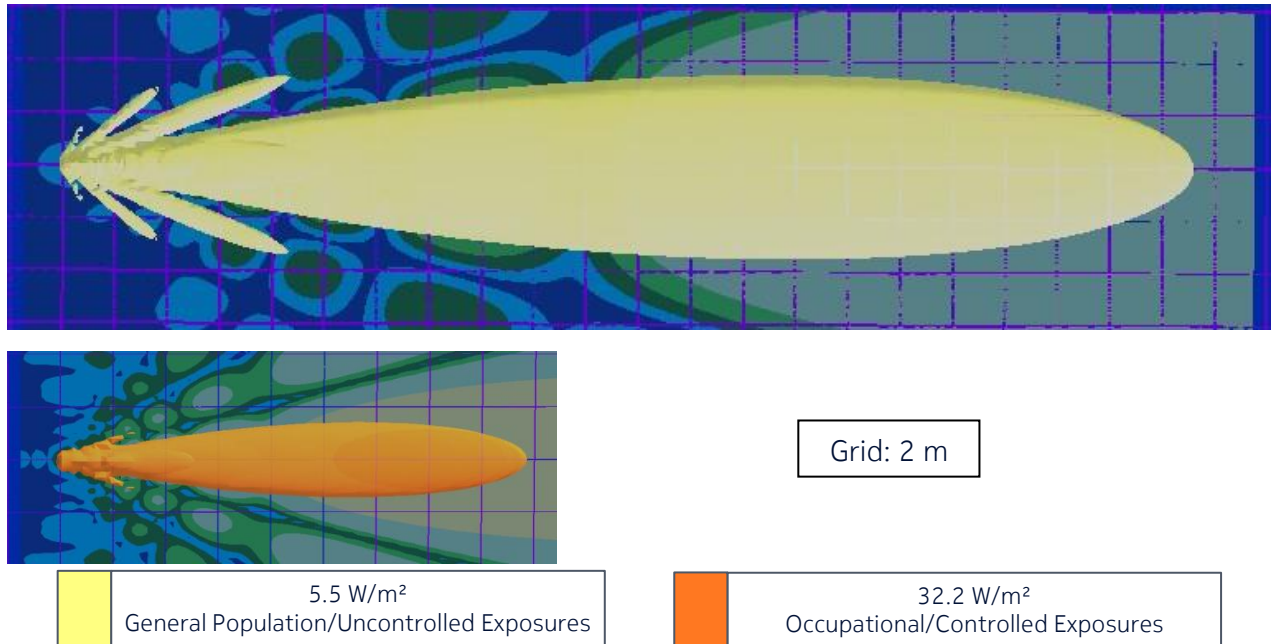
Figure 10 – Top view of the power density for the time-averaged maximum transmitted power of 424 W and beam oriented in azimuth = 0° & elevation = +6° with a gain of 24.8 (Canada)
