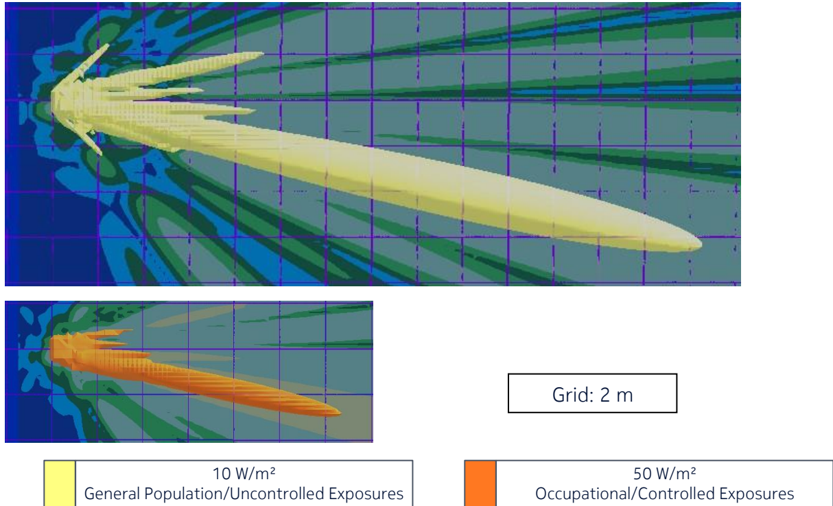
Figure 6 – Side view of the power density for the time-averaged maximum transmitted power of 424 W and beam oriented in azimuth = +3° & elevation = +13° with a gain of 24.0 dBi (EU/ICNIRP, Australia/NZ and US/related)
