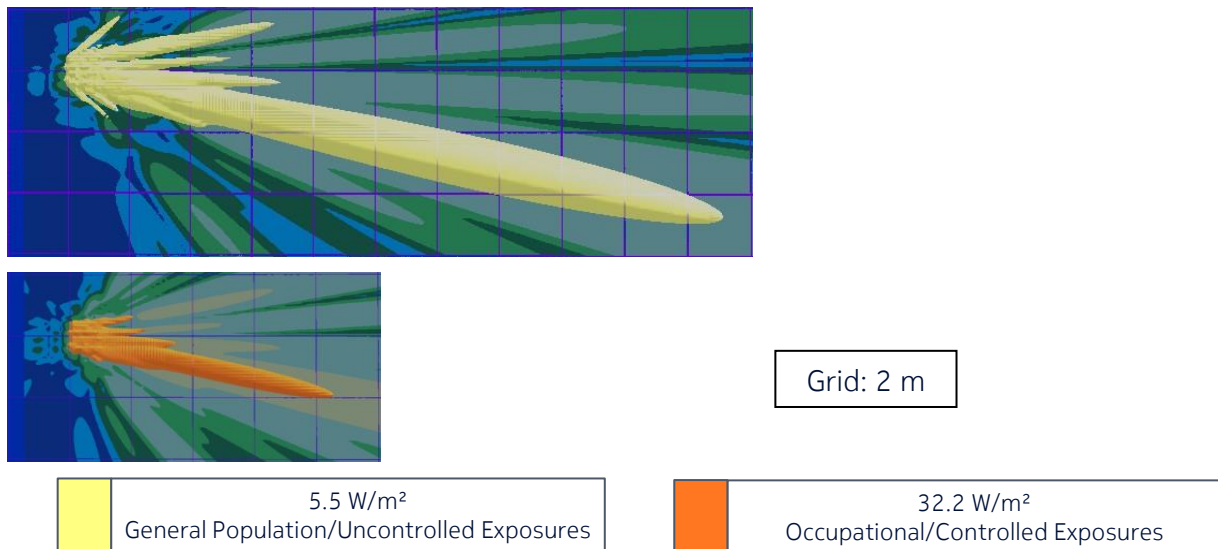
Figure 15 – Side view of the power density for the actual maximum transmitted power of 128 W (corresponding to the actual EIRP threshold of 75.1 dBm) and beam oriented in azimuth = +3° & elevation = +12° with a gain of 24.0 dBi (Canada)
