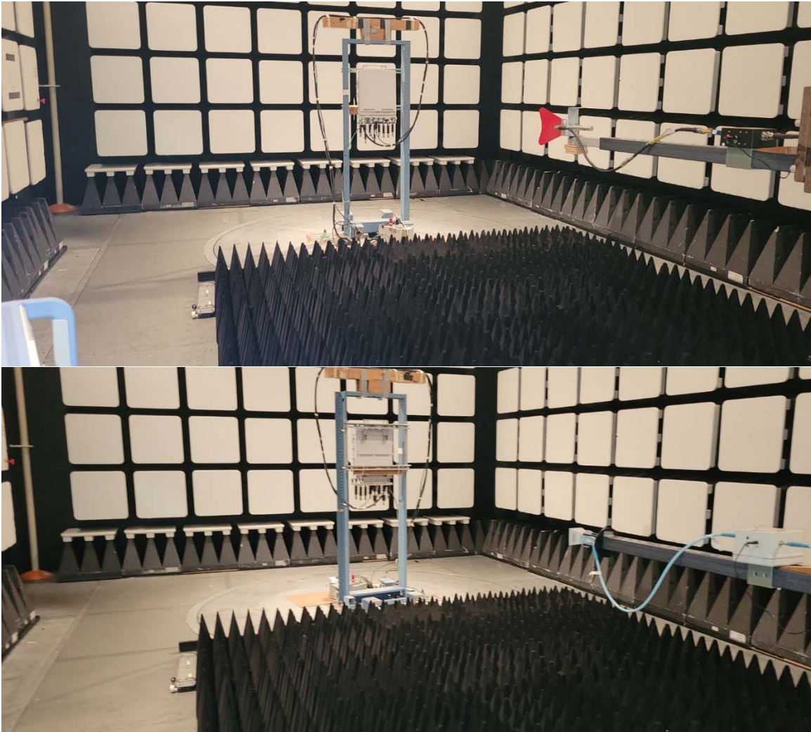
Figure 5. RADIATED EMISSIONS, 1 – 40 GHz
