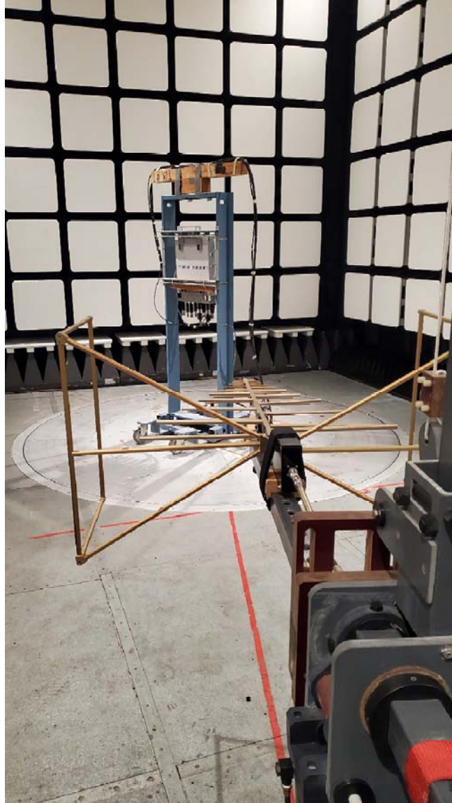
Figure 4. RADIATED EMISSIONS, 30 MHz – 1 GHz
