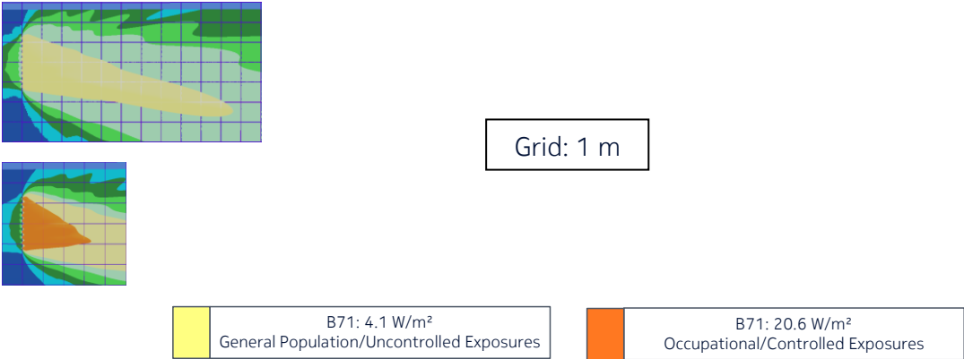
Figure 5 - Top view of the power density for the actual maximum transmitted power of 180 W in band B71 (corresponding to the actual EIRP threshold of 68.25 dBm) and the beam oriented in azimuth = 0° & elevation = +13° (US/related)
