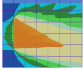
Figure 13 - Top view of the power density for the actual maximum transmitted power of 180 W in band B71 (corresponding to the actual EIRP threshold of 68.25 dBm) and the beam oriented in azimuth = 0° & elevation = +13° (Canada)
