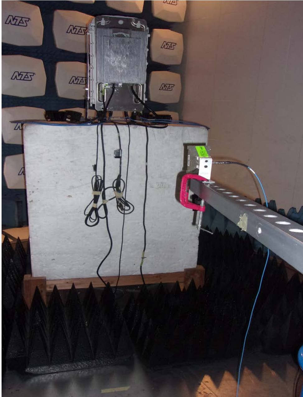
RE – 18-20GHz at 1m
