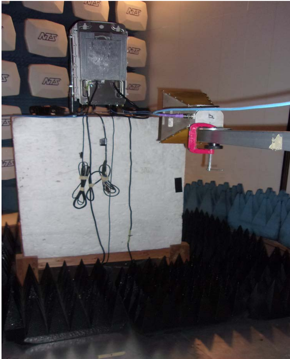
RE – 10-18GHz at 1m
