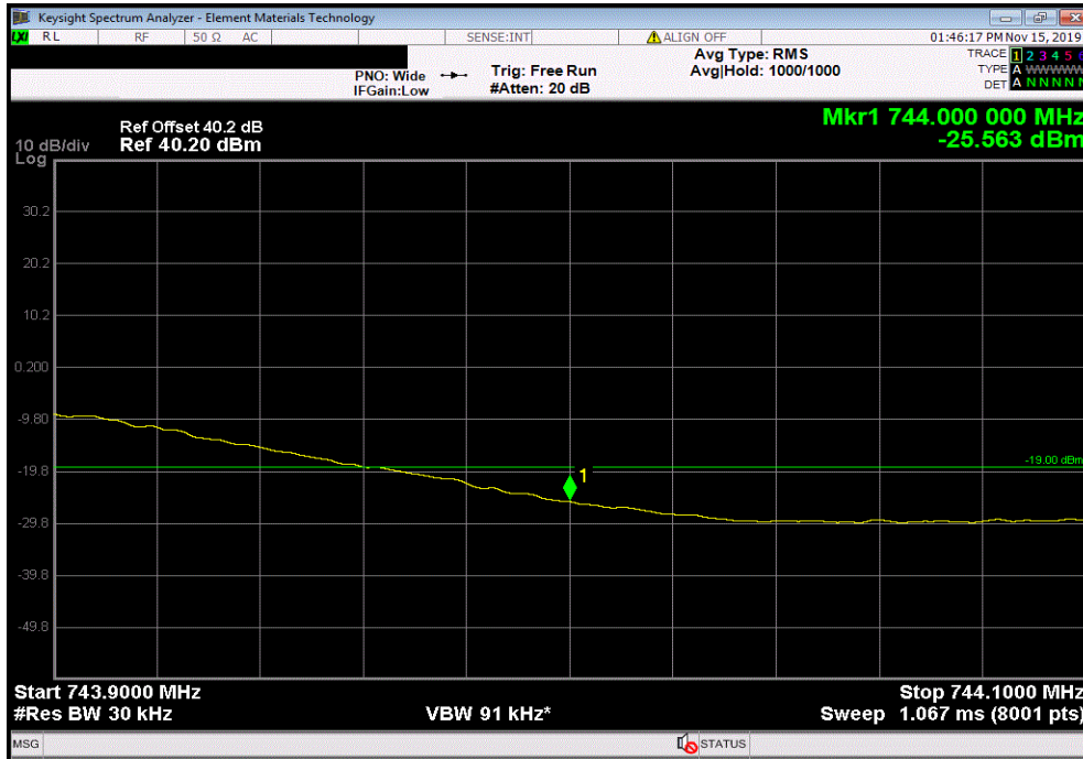
Band 12 Multicarrier, QPSK Modulation, Upper Band Edge, Measurement 2
