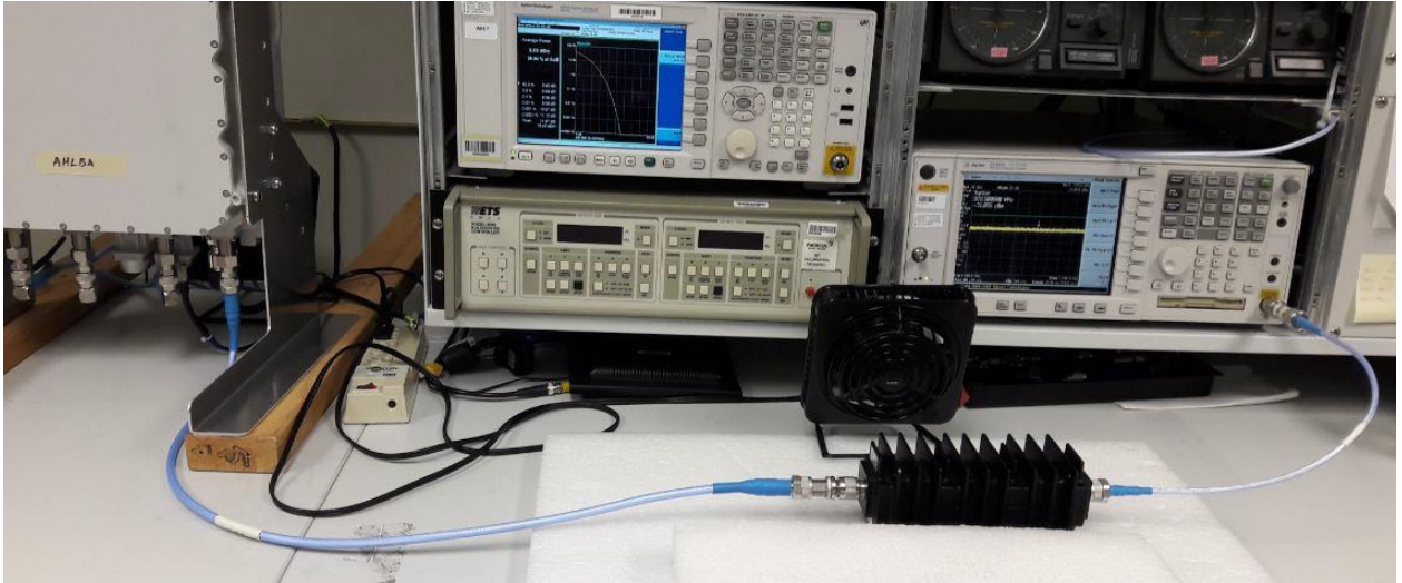
Photograph of 9kHz to 150kHz, 150kHz to 20MHz, 20MHz to 700MHz, 700MHz to 800MHz, and 800MHz to 1.1GHz Test Setup
