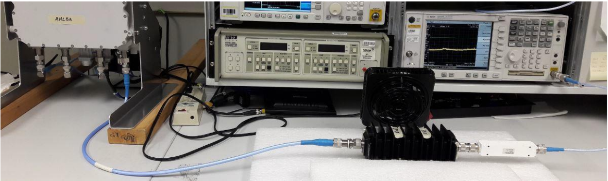
Photograph of 1.1GHz to 8GHz and 1559MHz to 1610MHz Test Setup
