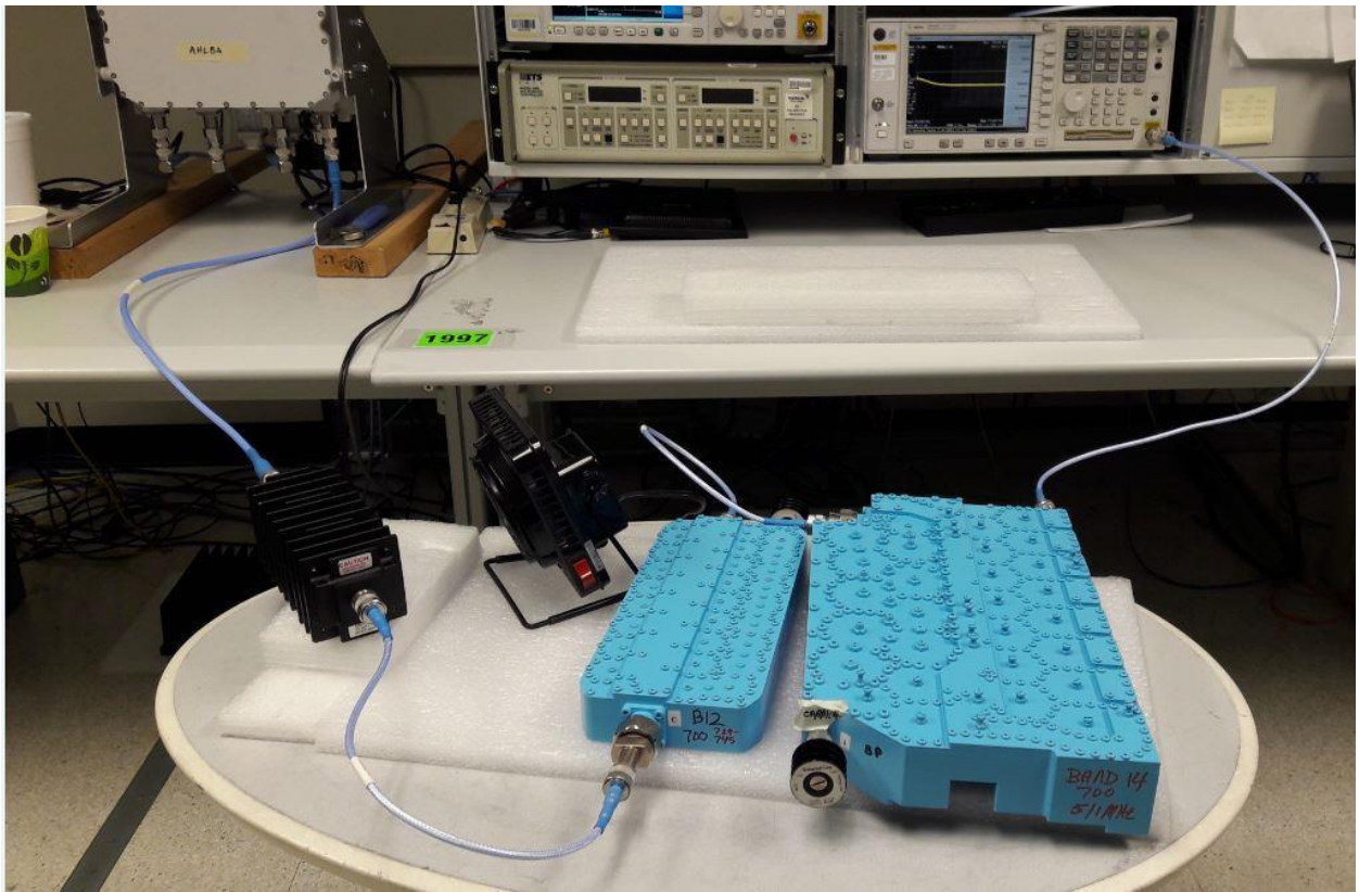
Photograph of 769MHz to 775MHz and 799MHz to 805MHz Test Setup
