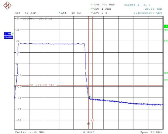
Figure 173 Spurious Emissions (Lower Band Edge) – QPSK (2120.0 MHz) (20MHz Channel BW)
