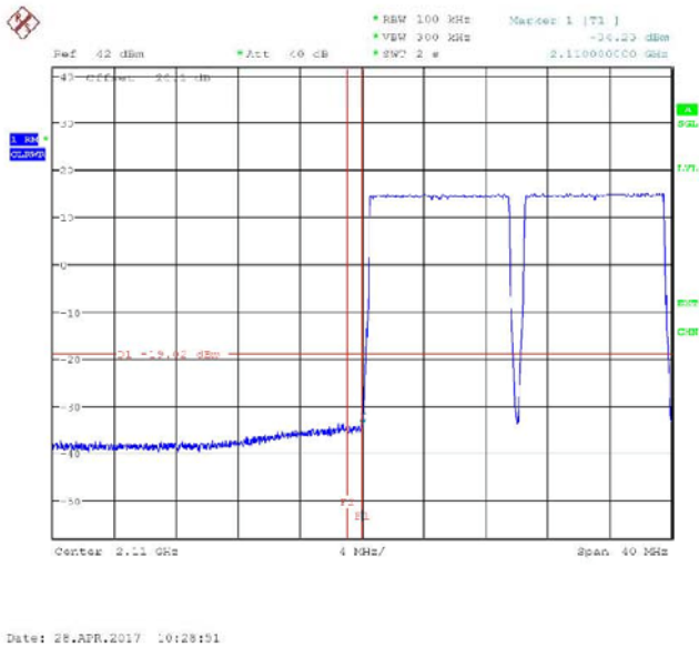
Figure 189 Spurious Emissions (Lower Band Edge) – QPSK (2115.0/2125.0 MHz) (10 MHz/10MHz Channel BW)
