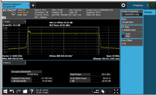
64QAM / Chain 0
