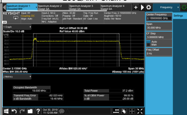
256QAM / Chain 3
