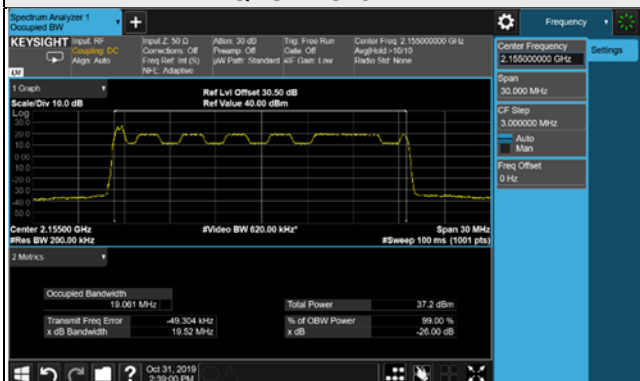
64QAM / Chain 0
