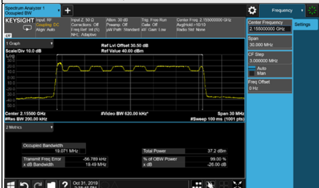
64QAM / Chain 2
