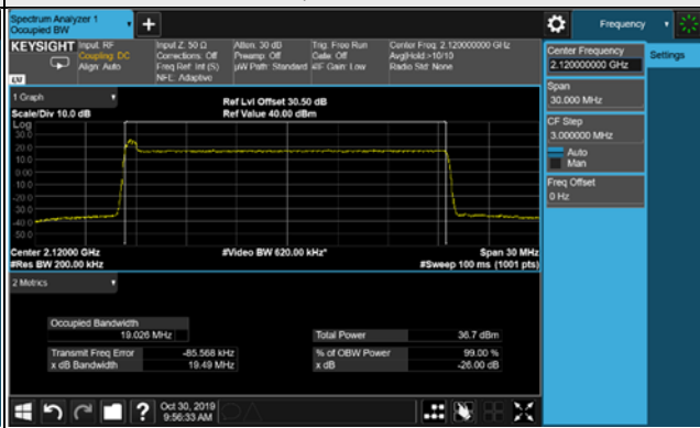
256QAM / Chain 0
