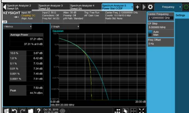
64QAM / Chain 0
