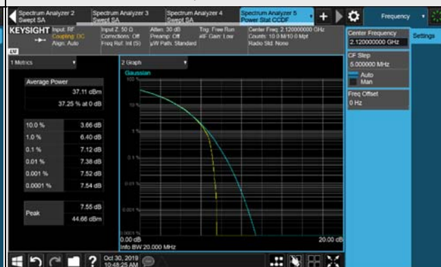
256QAM / Chain 1
