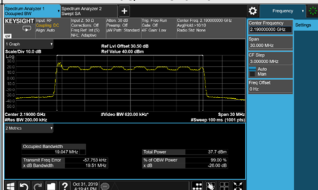
256QAM / Chain 0
