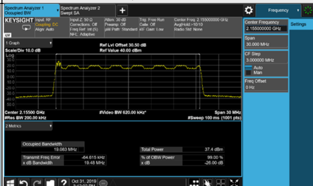
256QAM / Chain 3
