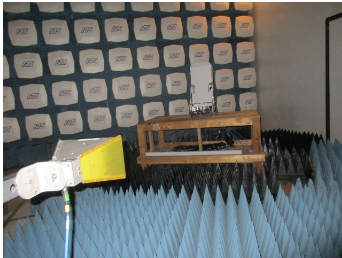
RE – 1-10GHz at 3m
