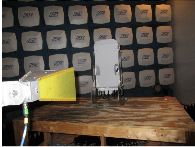
RE – 10-18GHz at 1m
