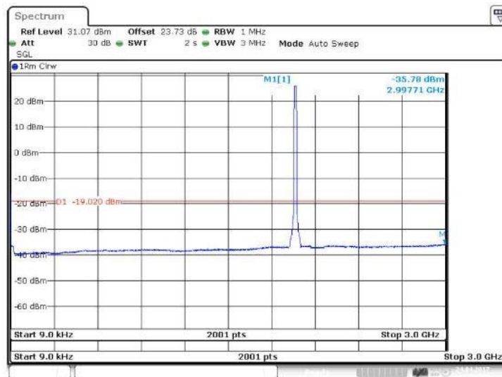
Figure 47 Spurious Emissions (9kHz – 3GHz) - QPSK (1962.5 MHz) (20MHz Channel BW)
