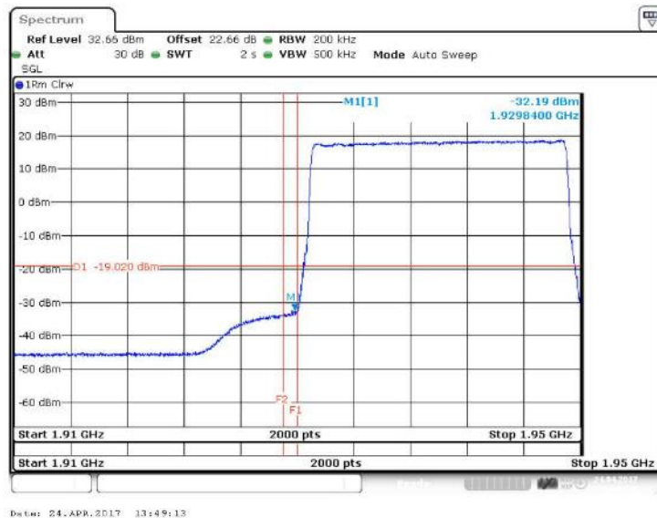
Figure 41 Spurious Emissions (Lower Band Edge) – 256QAM (1940.0 MHz) (20MHz Channel BW)
