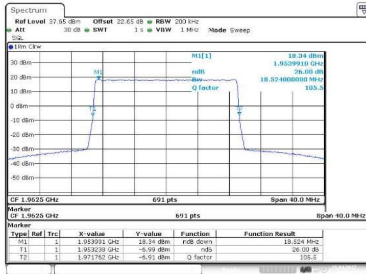
Figure 19 Occupied Bandwidth – 64QAM (1962.5 MHz) (20MHz Channel BW)
