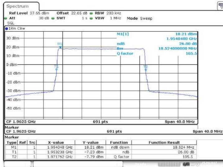
Figure 25 Occupied Bandwidth – QPSK (1962.5 MHz) (20MHz Channel BW)
