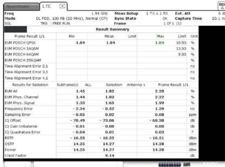
Figure 6 I/Q constellation table with I/Q error – QPSK (1940.0 MHz) (20MHz Channel BW)
