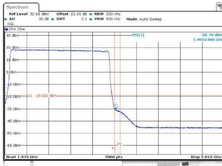
Figure 38 Spurious Emissions (Upper Band Edge) – 64QAM (1985.0 MHz) (20MHz Channel BW)
