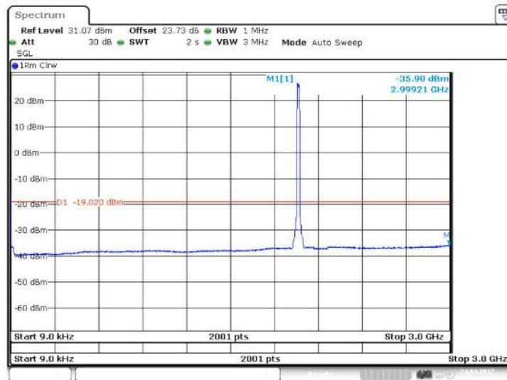
Figure 34 Spurious Emissions (Upper Band Edge) – 16QAM (1985.0 MHz) (20MHz Channel BW)
