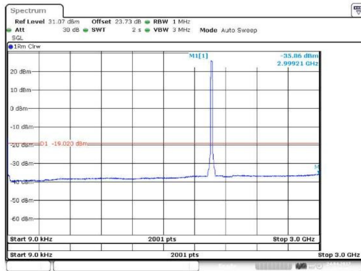
Figure 30 Spurious Emissions (Upper Band Edge) – QPSK (1985.0 MHz) (20MHz Channel BW)
