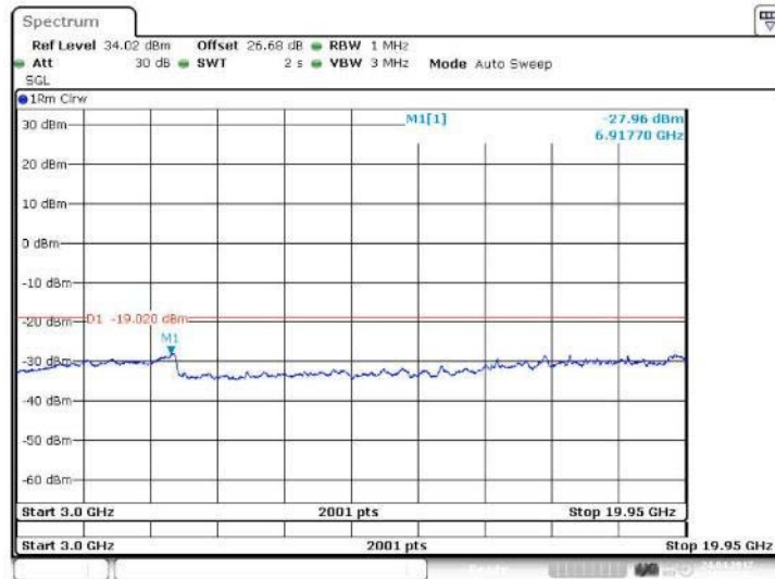
Figure 44 Spurious Emissions (3GHz – 19.950GHz) – 256QAM (1962.5 MHz) (20MHz Channel BW)
