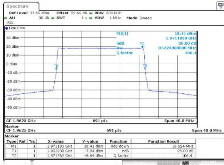
Figure 19 Occupied Bandwidth – 64QAM (1962.5 MHz) (20MHz Channel BW)
