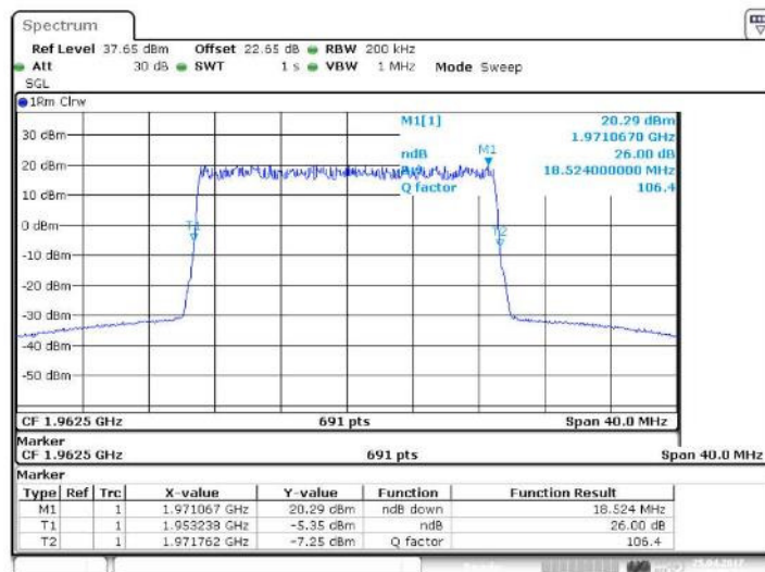
Figure 13 Occupied Bandwidth – QPSK (1962.5 MHz) (20MHz Channel BW)
