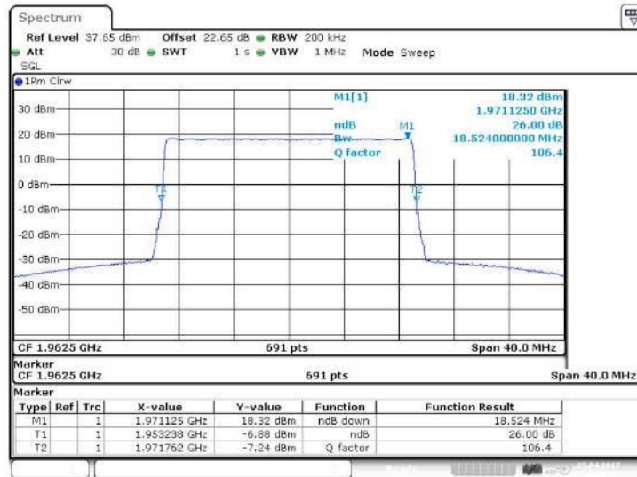
Figure 17 Occupied Bandwidth – QPSK (1962.5 MHz) (20MHz Channel BW)
