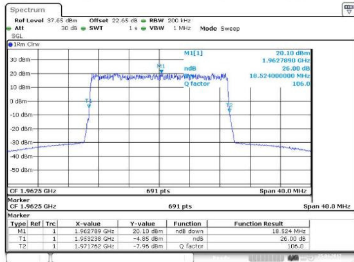
Figure 17 Occupied Bandwidth – QPSK (1962.5 MHz) (20MHz Channel BW)
