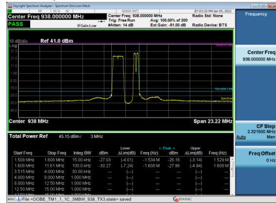
TM 1.1 / QPSK / 938.0MHz / 1.4+0.2+0.2MBW / TX3
