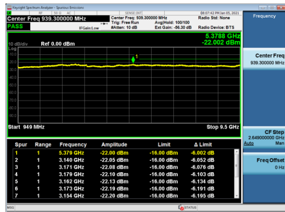
949MHz – 9.5GHz
