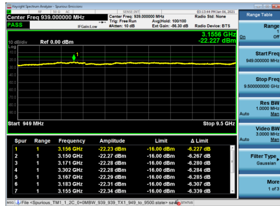
949MHz – 9.5GHz
