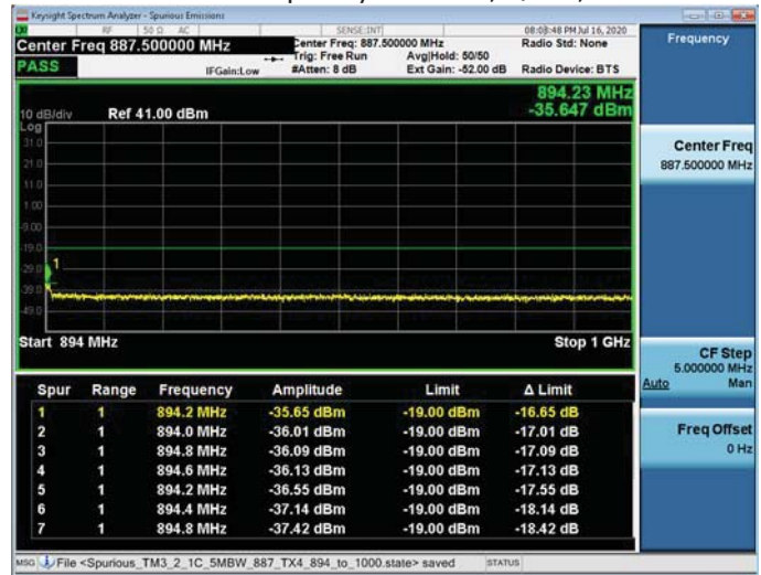
894MHz – 1GHz Channel Frequency 887MHz, QPSK, TX4
