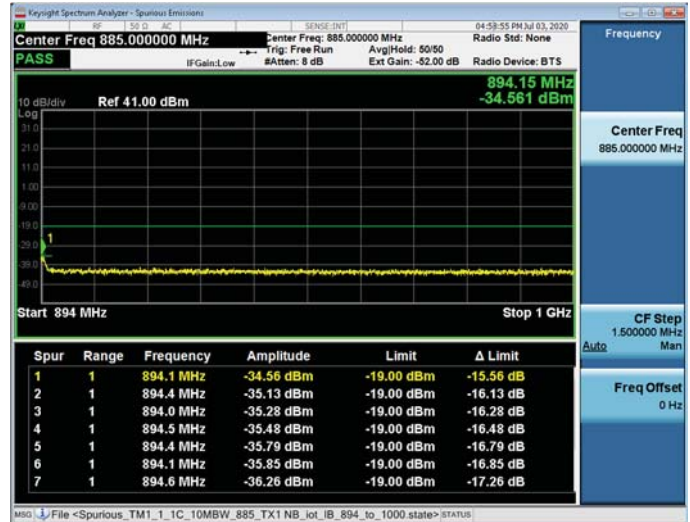
894MHz – 1GHz
