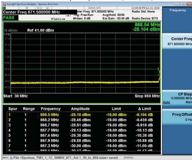
30MHz – 869MHz Channel Frequency 871MHz, 64QAM, TX1
