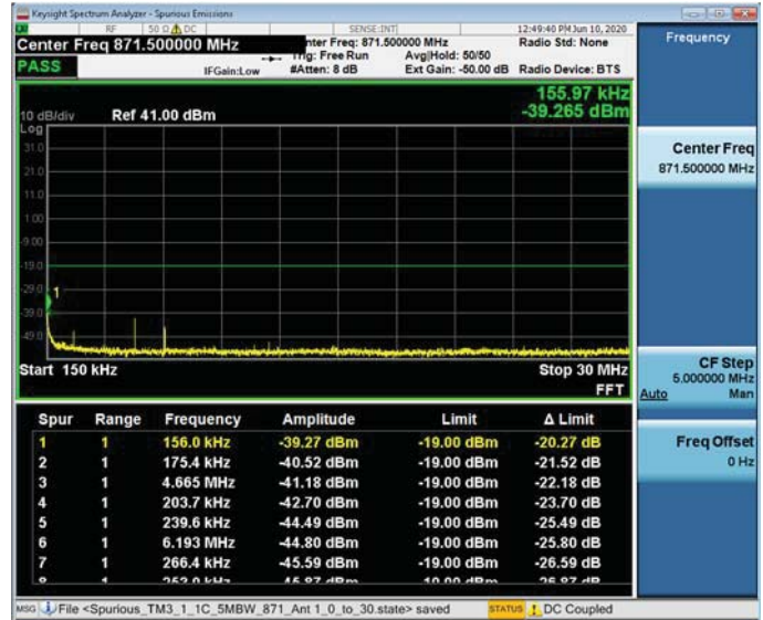
150kHz – 30MHz Channel Frequency 871MHz, 64QAM, TX1
