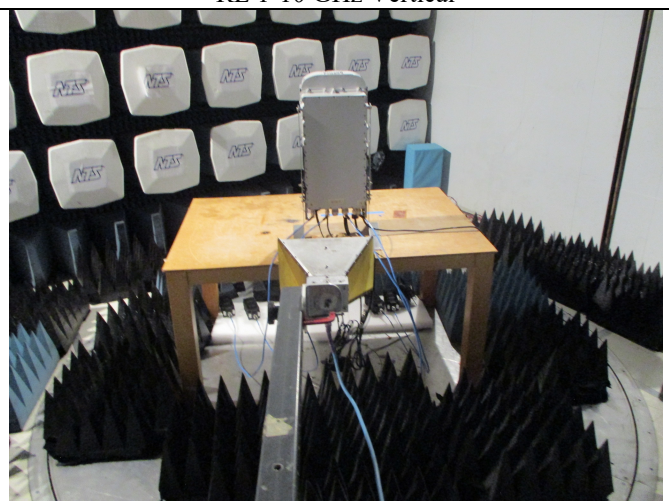
RE 10-18 GHz Vertical
