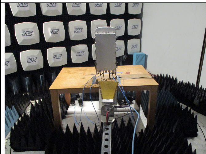
RE 10-18 GHz Horizontal
