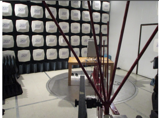
RE 30-1000 MHz Vertical
