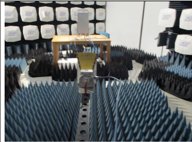
RE 1-10 GHz Horizontal
