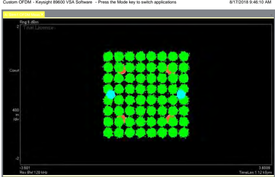
Sample 64QAM 27.6 GHz Vertical Polarization
