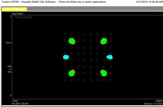
Sample QPSK 27.6GHz Vertical Polarization
