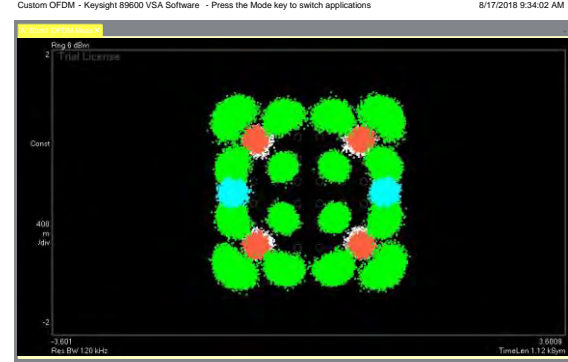
Sample 16QAM 27.6 GHz Horizontal Polarization
