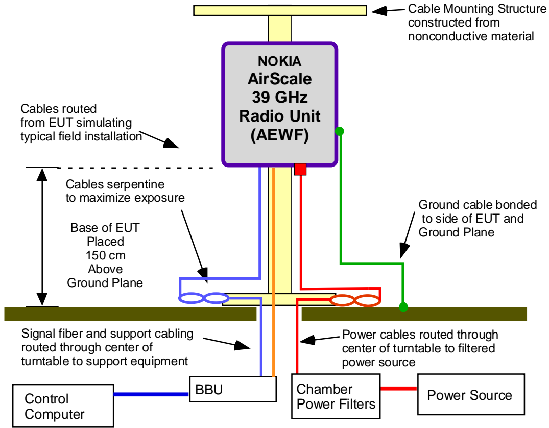
Figure 4.5 Radiated Emissions Product Setup Radiated Emissions Setup Nokia AirScale 39 GHz Radio Unit (AEUA)
