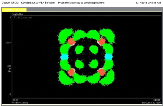
Sample 16QAM 27.6 GHz Vertical Polarization
