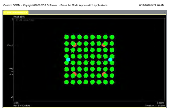
Sample 64QAM 27.6 GHz Horizontal Polarization
