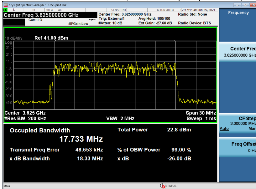
Single Carrier - 8-Beam 32T32R 20 MHz Test Model 1.1, Modulation QPSK, Channel Frequency 3625MHz, TX3
