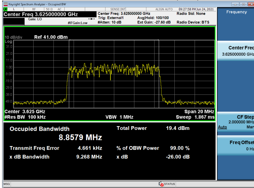
Single Carrier - 8-Beam 32T32R 10 MHz Test Model 1.1, Modulation QPSK, Channel Frequency 3625MHz, TX3
