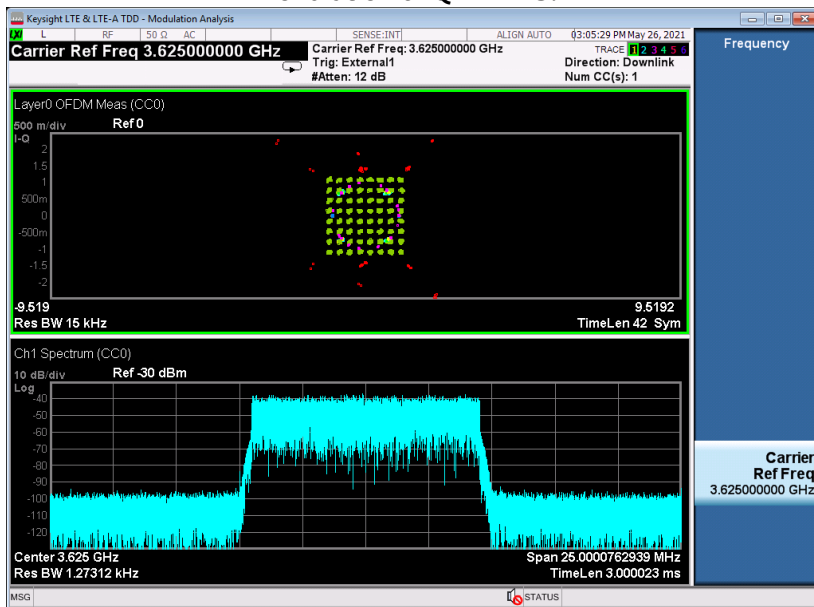
Modulation 64QAM TM3.1
