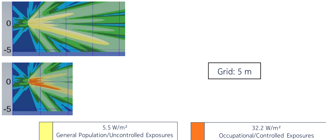
Figure 11 – Side view of the power density for the time-averaged actual maximum transmitted power of 85 W and the beam oriented in azimuth = -5^\circ & elevation = +15^\circ (Canada)
