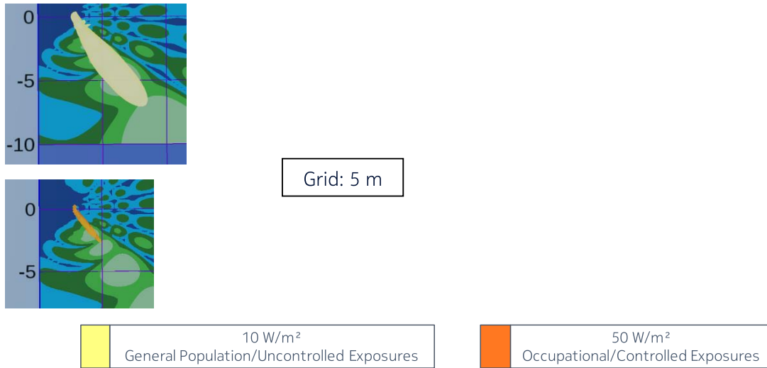
Figure 7 – Top view of the power density for the time-averaged actual maximum transmitted power of 85 W and the beam oriented in azimuth = -51^\circ & elevation = +4^\circ (EU/ICNIRP, Australia/NZ and US/related)
