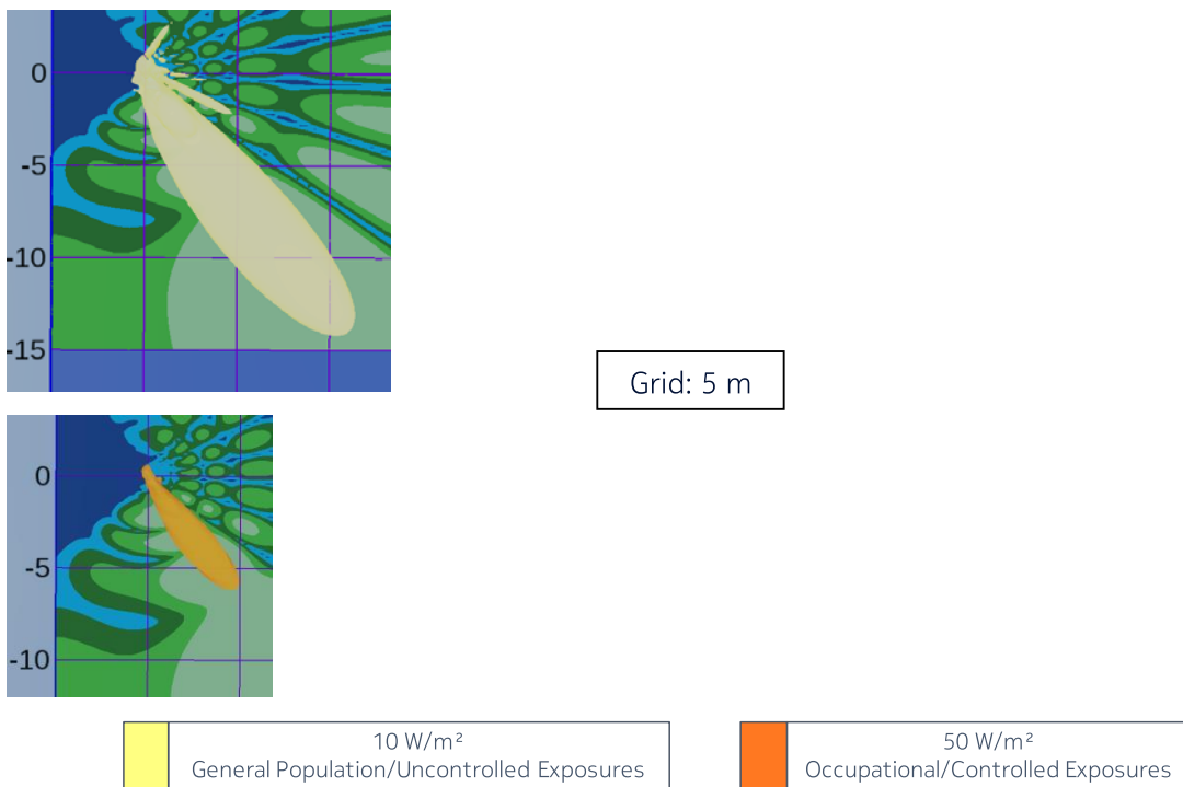
Figure 6 – Top view of the power density for the time-averaged maximum transmitted power of 339 W and the beam oriented in azimuth = -51^\circ & elevation = +4^\circ (EU/ICNIRP, Australia/NZ and US/related)
