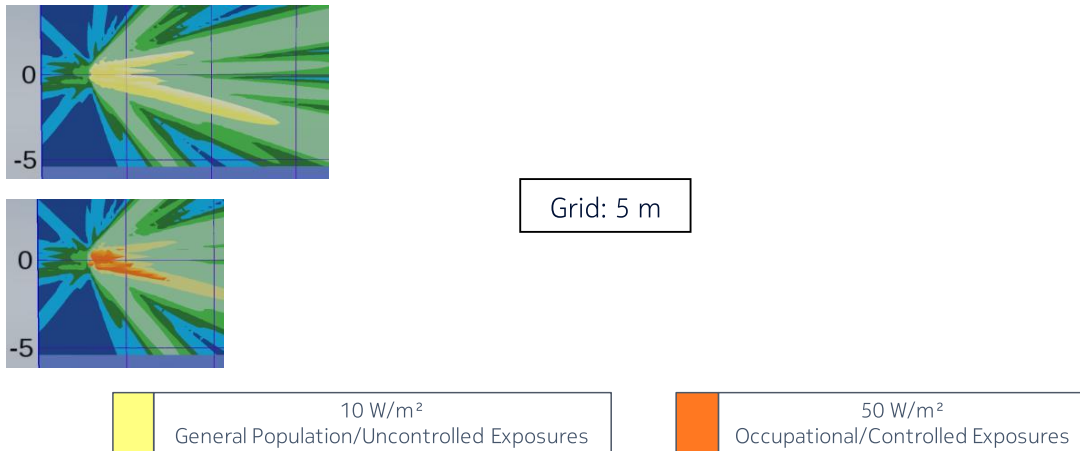
Figure 5 – Side view of the power density for the time-averaged actual maximum transmitted power of 85 W and the beam oriented in azimuth = -5^\circ & elevation = +15^\circ (EU/ICNIRP, Australia/NZ and US/related)
