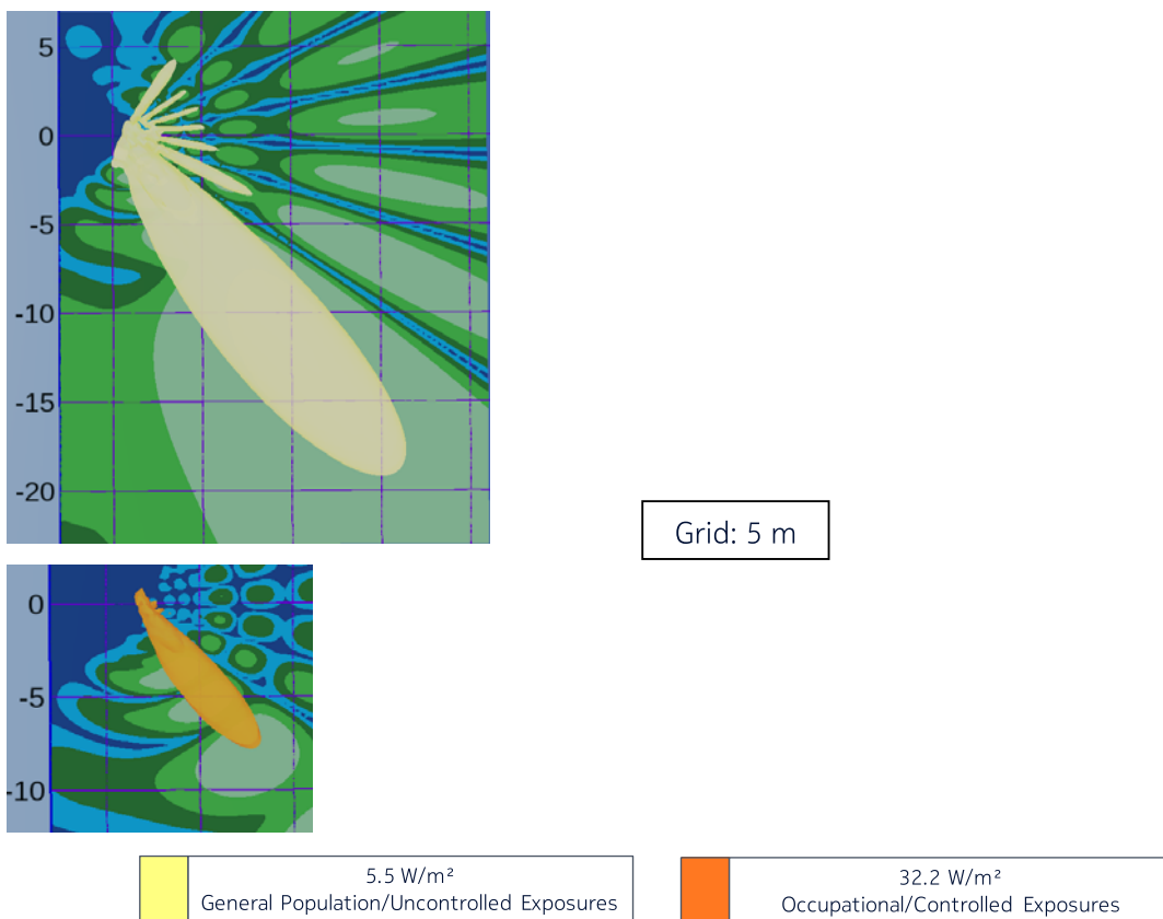
Figure 12 – Top view of the power density for the time-averaged maximum transmitted power of 339 W and the beam oriented in azimuth = -51^\circ & elevation = +4^\circ (Canada)
