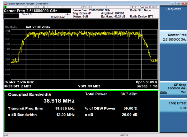
256QAM, 40MBW, 2516
