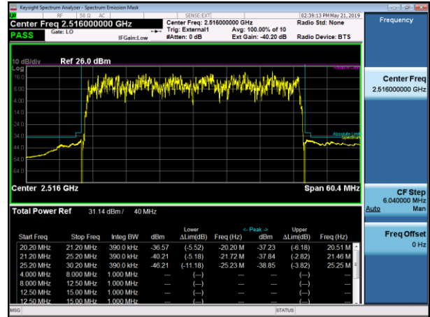
QPSK+16QAM, 40MBW, 2516
