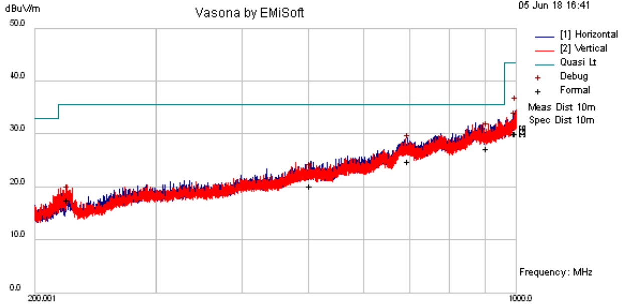
Radiated Emissions Template: RDE AR8 10M 30MHz-1GHz VCCI Filename: c:\program files\emisoft - vasona\results\2018-0080 aahe mmimo - full band\T12 RE200M-1G 64Atten FCCB 10M.emi
