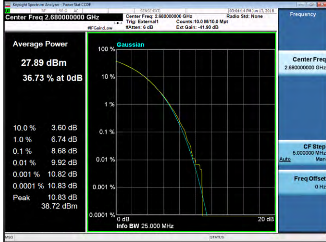
PAR, AAHE mMIMO - B41, 1C, 28dBm, 20MBW, TM3.1A, 2680 MHz.
