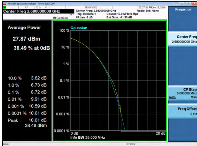
PAR, AAHE mMIMO - B41, 1C, 28dBm, 20MBW, TM3.2, 2680 MHz.
