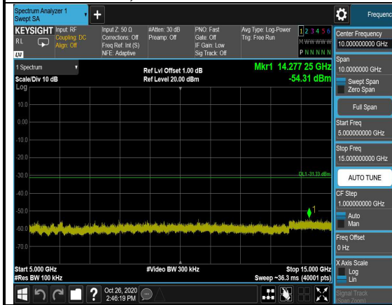
802.11n(HT40),2452MHz,Ant0,Plot 1,Reference Level
