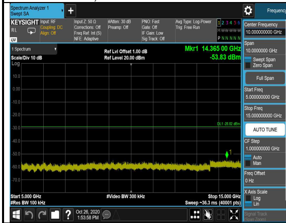
802.11n(HT20),2462MHz,Ant0,Plot 1,Reference Level
