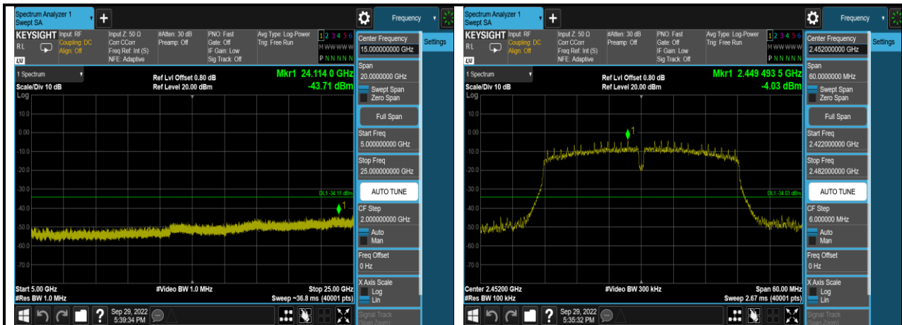
802.11n(HT40),2452MHz,Ant0,Plot 2,Band Edge
