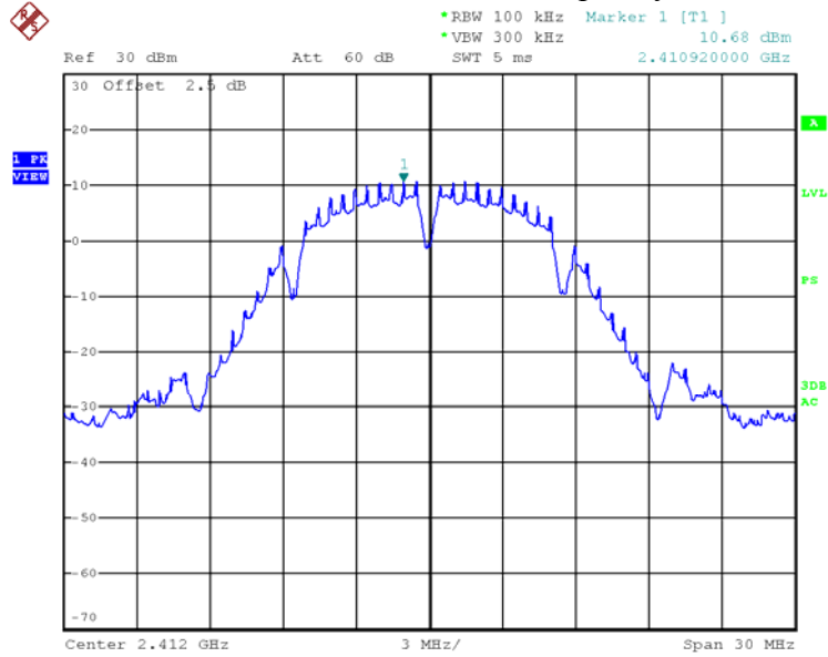
Reference Level – Frequency L
