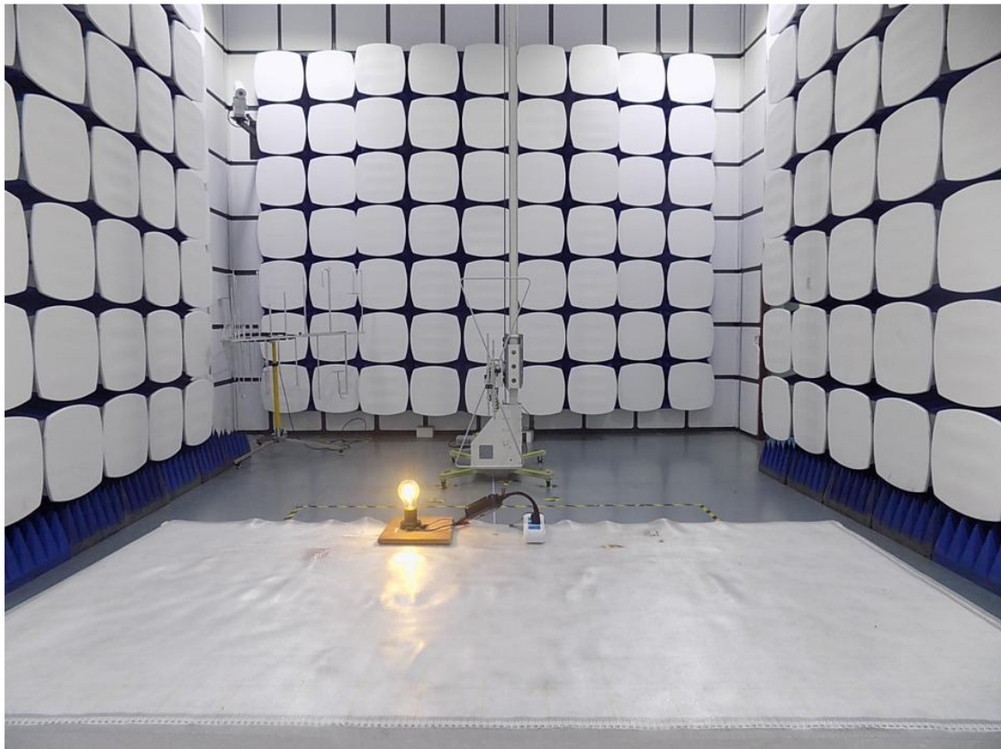
1.Setup for Radiated Emission below 1GHz
