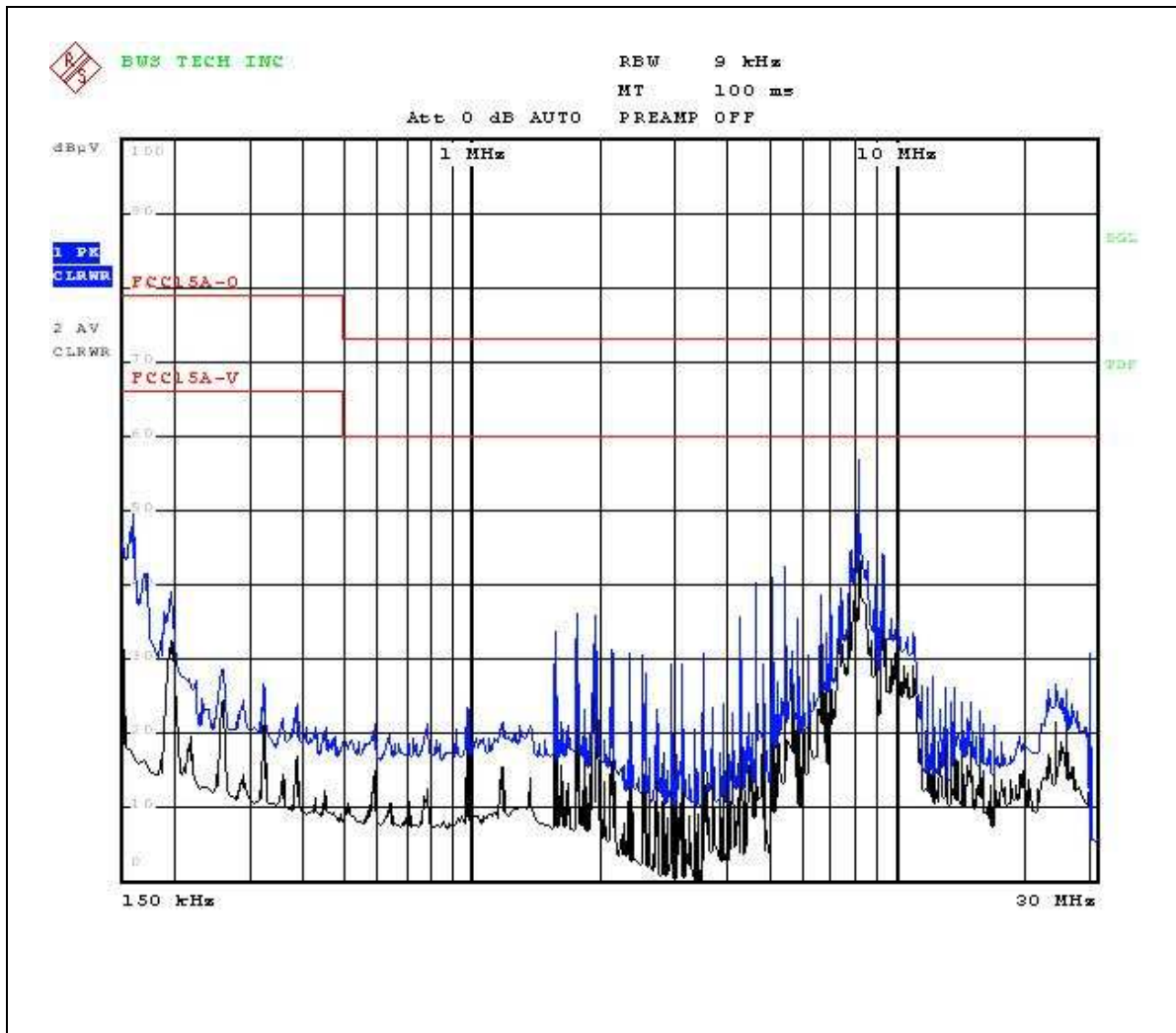
Figure 3 Conducted Emissions Graph – Up link mode , Line Polarity : Neutral
