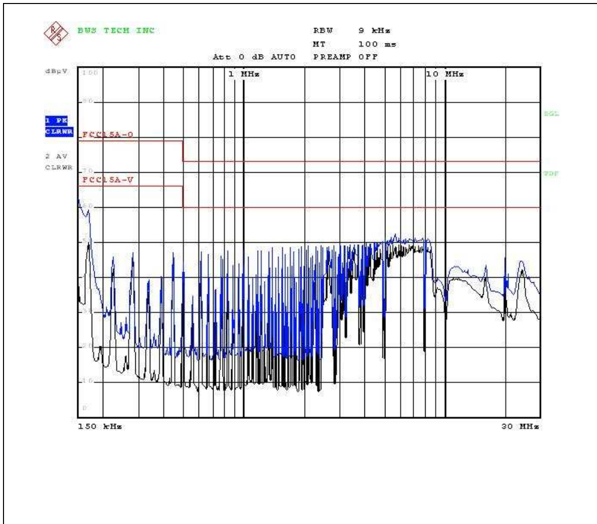
Figure 2 Conducted Emissions Graph – Up link mode , Line Polarity : Hot
