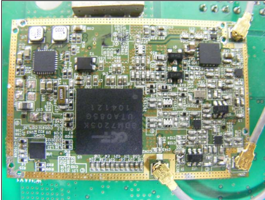
PCB top view (Wimax Module Board)
