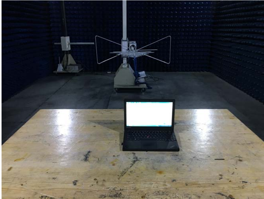
Photograph of set-up for Radiated Emission below 1000MHz
