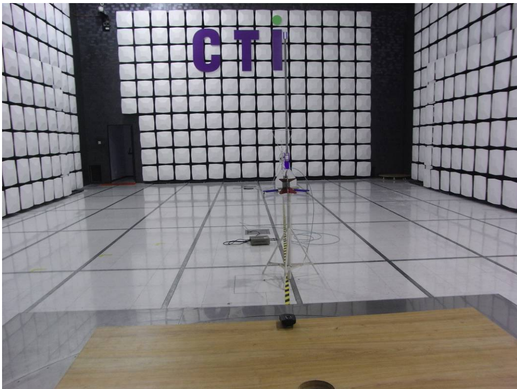
TEST SETUP OF RADIATED EMISSION (1GHz-25GHz)
