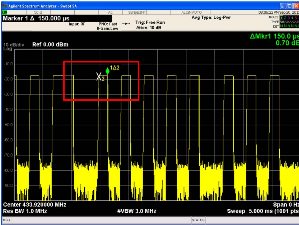
Duration Time of Type 1 (2 nd Data) : 150.0 μs
