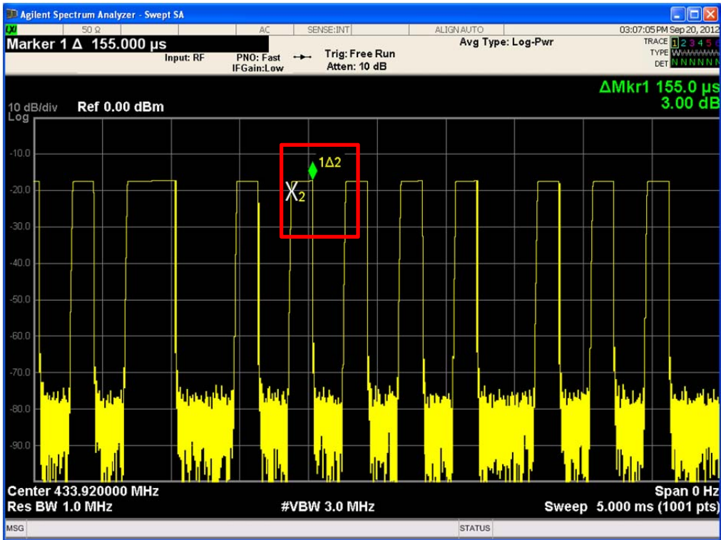
Duration Time of Type 2 (Bit 0) : 155.0 \mu s
