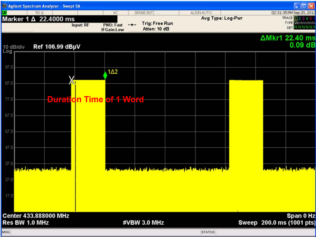
Duration Time of 1 word : 22.40 ms
