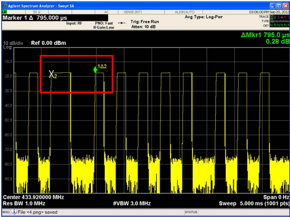
Period of Type 1 (1 st Data) : 795.0 μs
