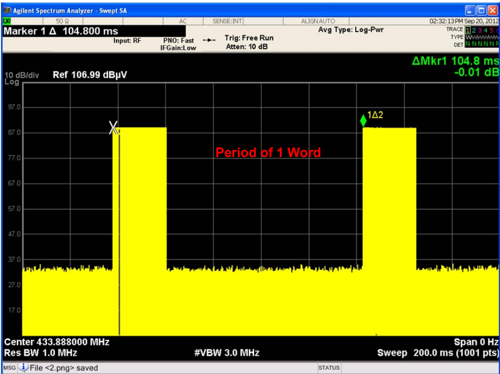
Period of 1 word : 104.80 ms
