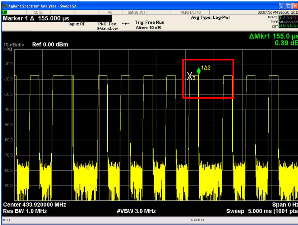
Duration Time of Type 3 (Bit 1) : 155.0 μs
