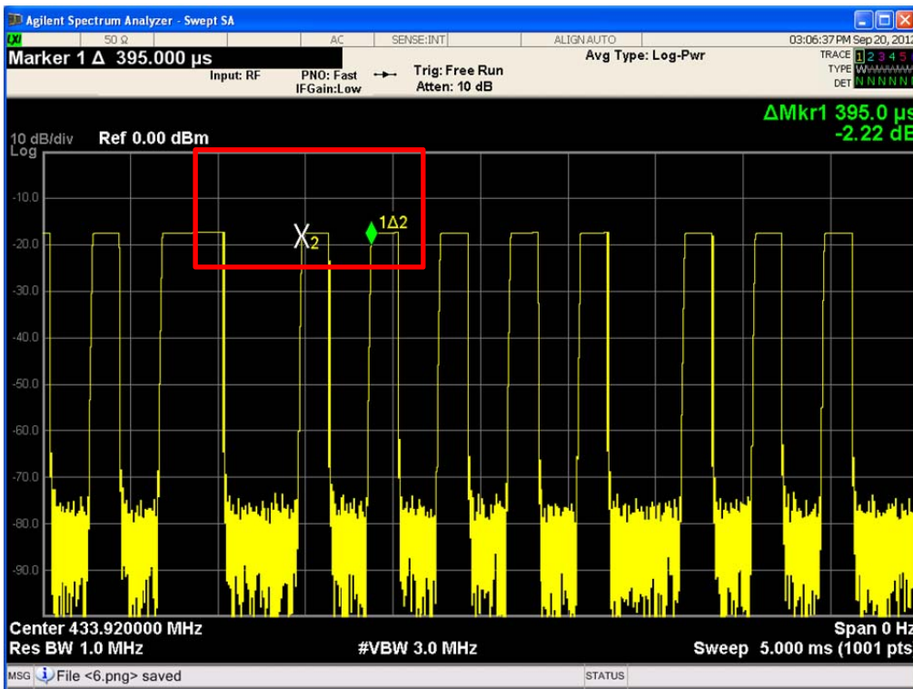
Period of Type 1 (2 nd Data) : 395.0 μs
