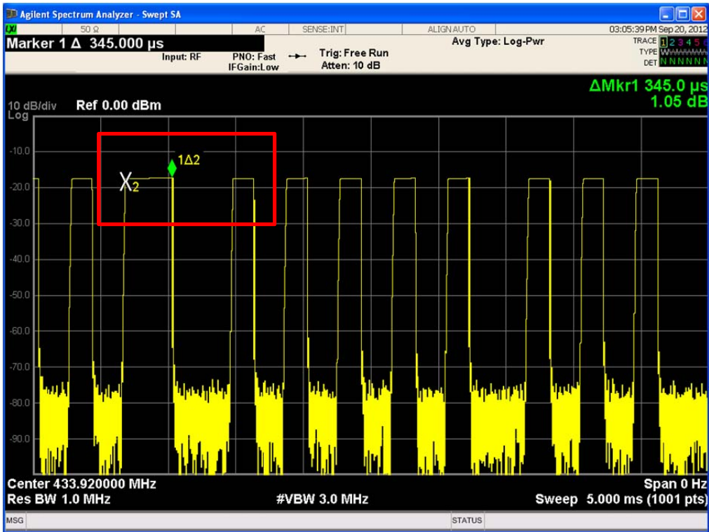
Duration Time of Type 1 (1 st Data) : 345.0 μs
