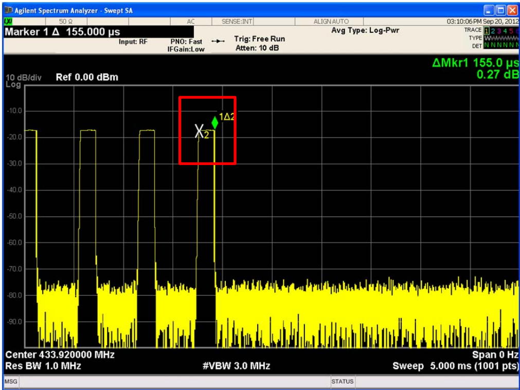
Duration Time of Type 4 (Bit 0) : 155.0 μs
