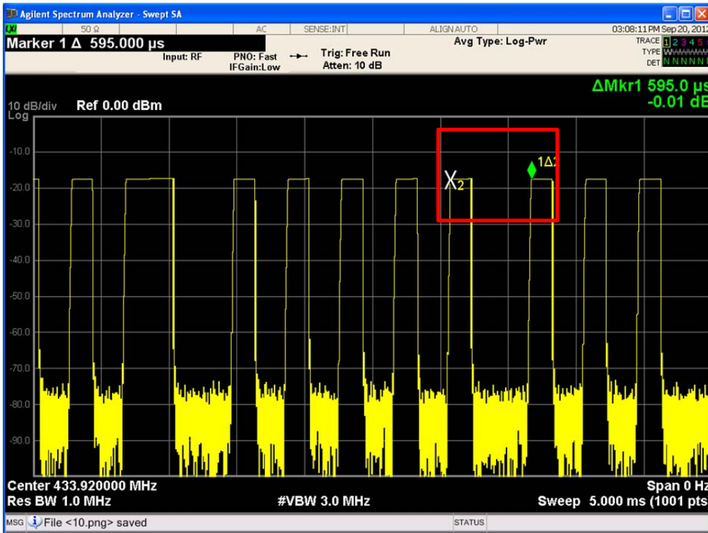
Period of Type 3 (Bit 1) : 595.0 μs
