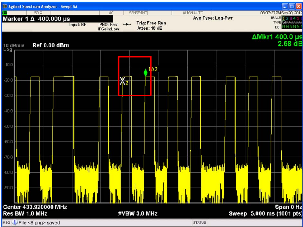
Period of Type 2 (Bit 0) : 400.0 \mu s
