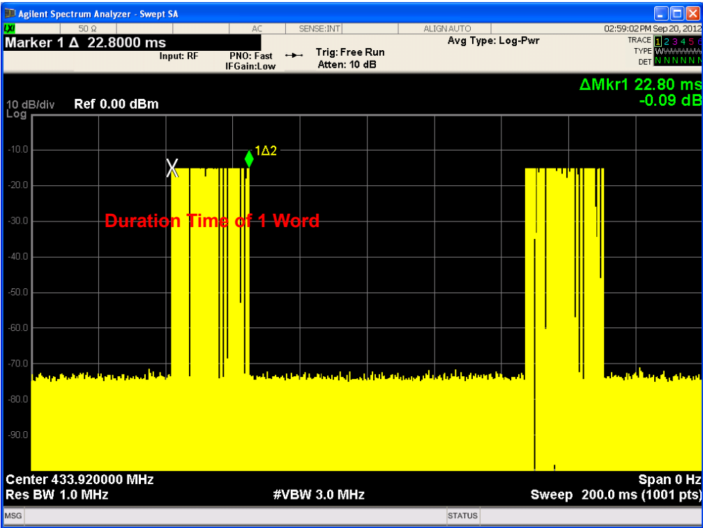
Duration Time of 1 word : 22.80 ms
