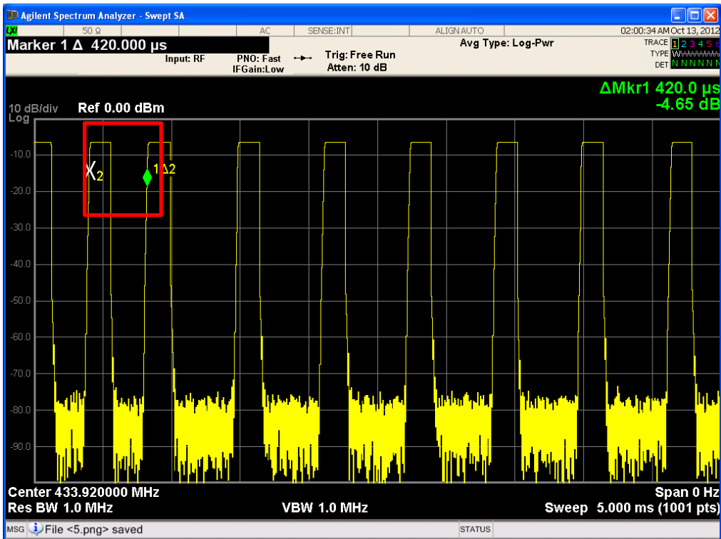
Period of Type 2 (Bit 0) : 420.0 μs
