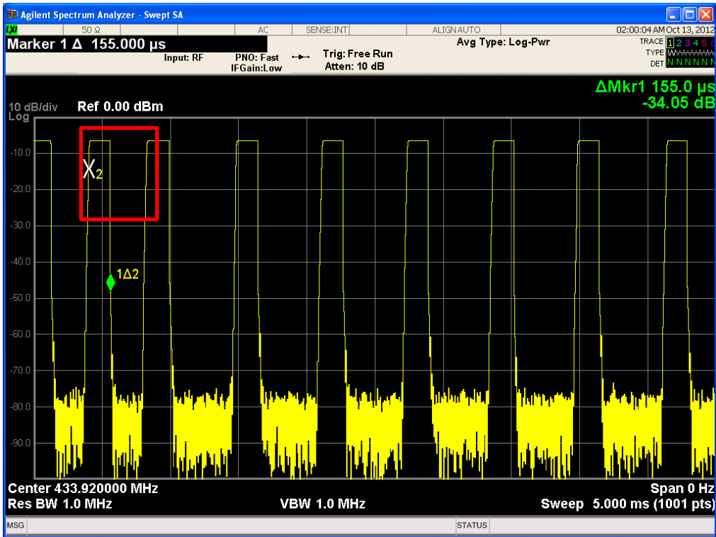
Duration Time of Type 2 (Bit 0) : 155.0 μs
