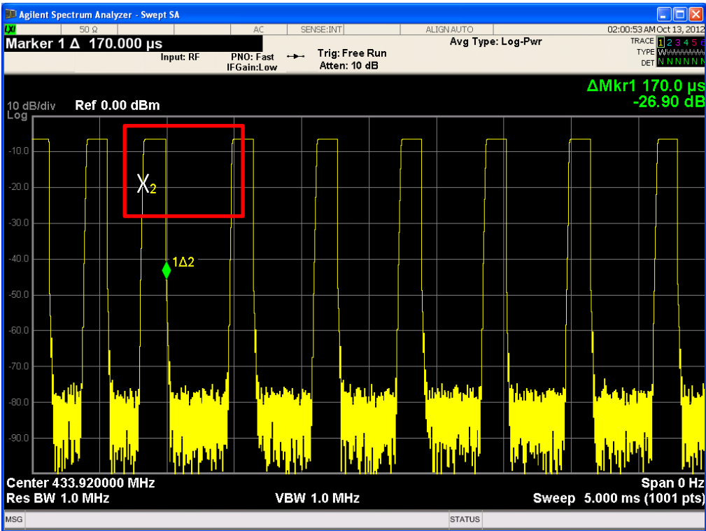
Duration Time of Type 3 (Bit 1) : 170.0 μs
