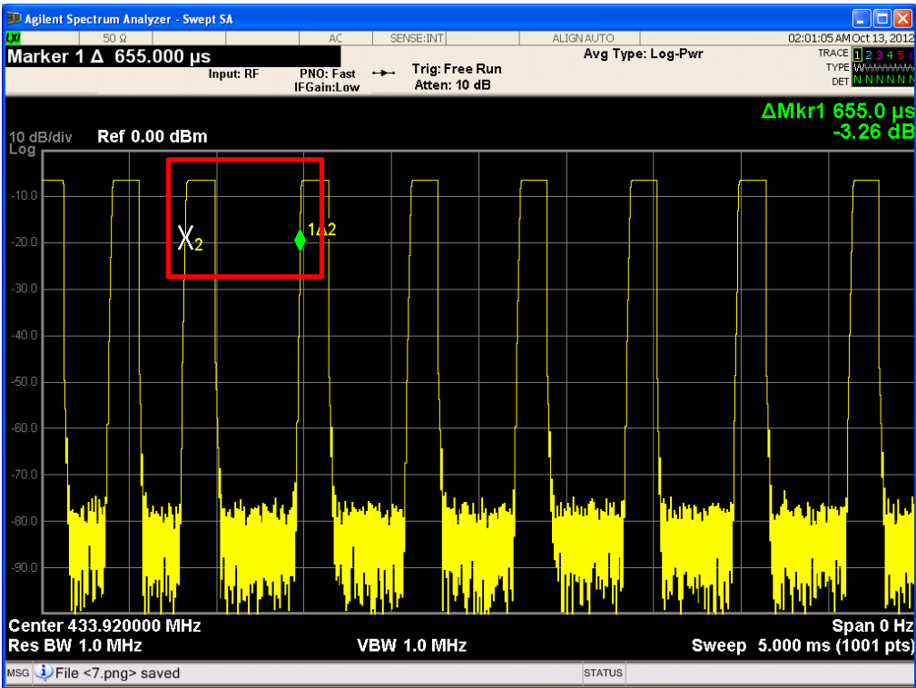
Period of Type 3 (Bit 1) : 655.0 μs
