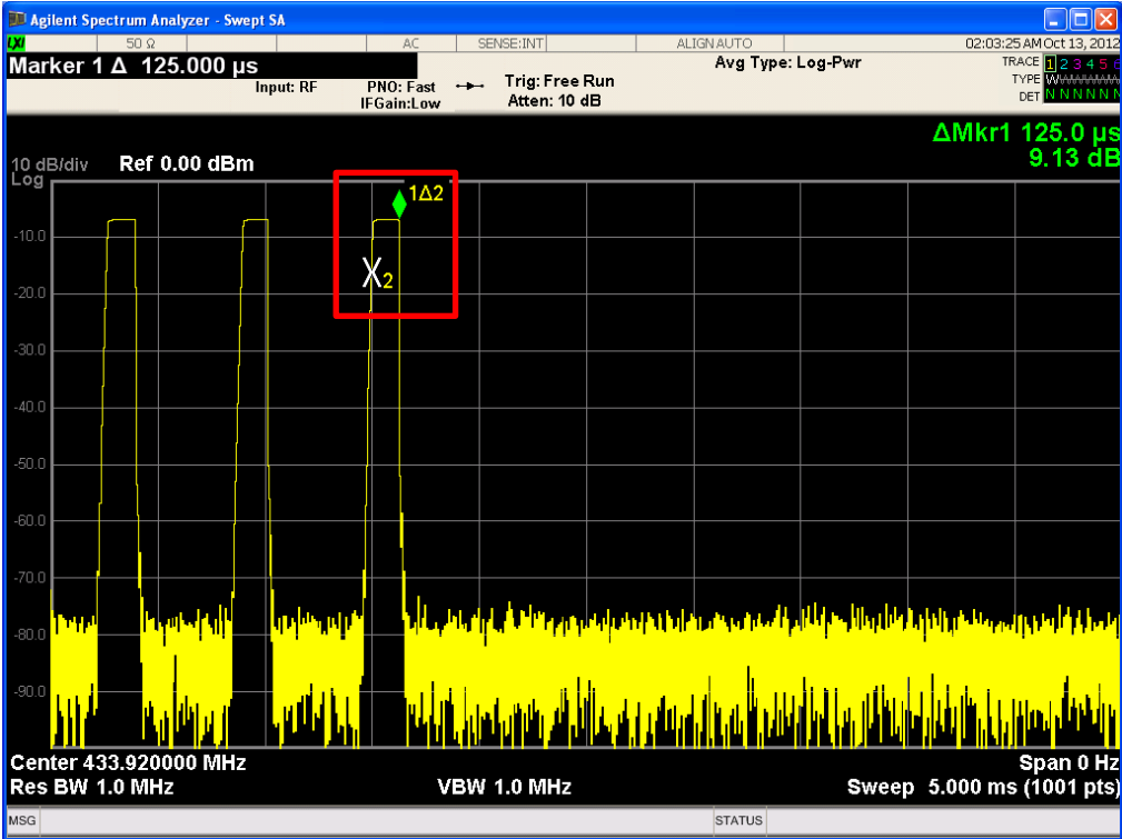
Duration Time of Type 4 (Bit 0) : 125.0 μs
