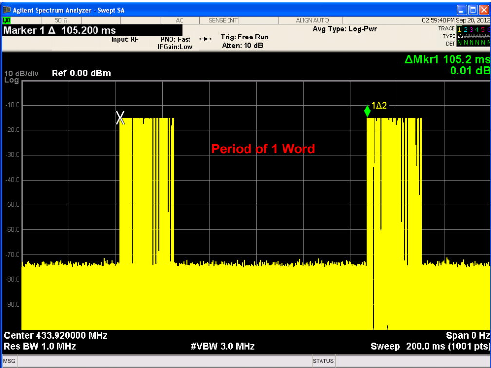
Period of 1 word : 105.20 ms
