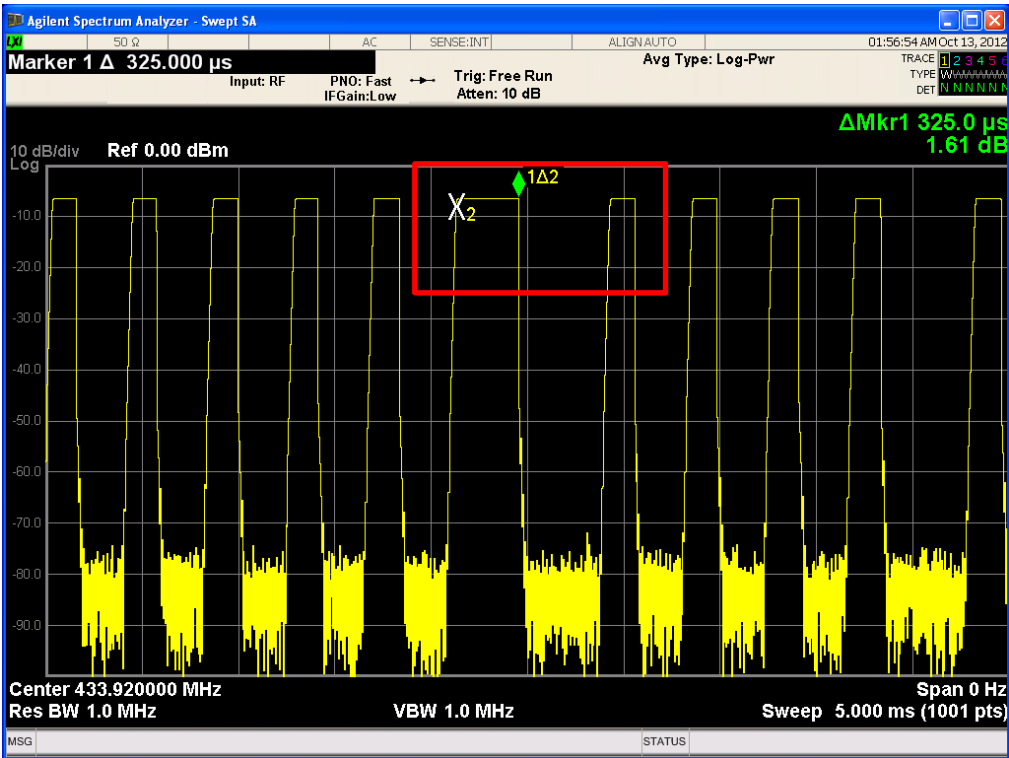
Duration Time of Type 1 (1 st Data) : 325.0 μs
