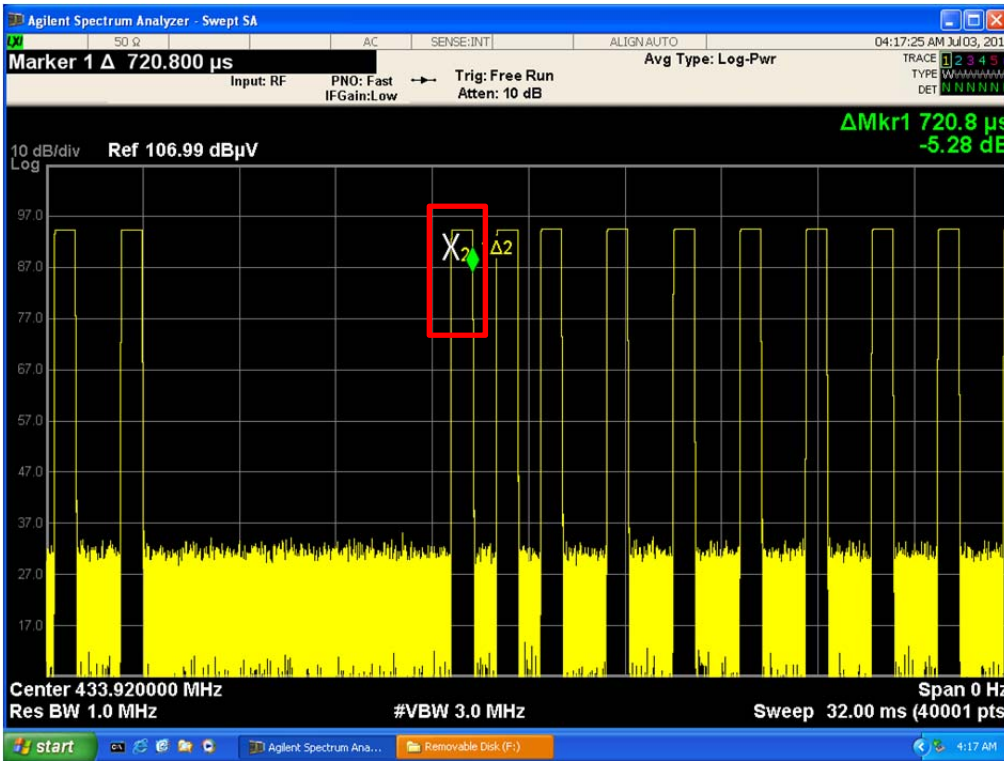
Duration Time of Type 2 (Bit 0) : 720.8 μs
