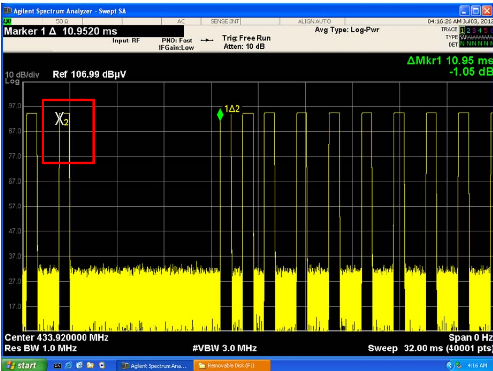
Period of Type 1 (SYNC) : 10 950 μs
