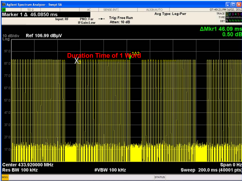
Duration Time of 1 word : 46.09 ms
