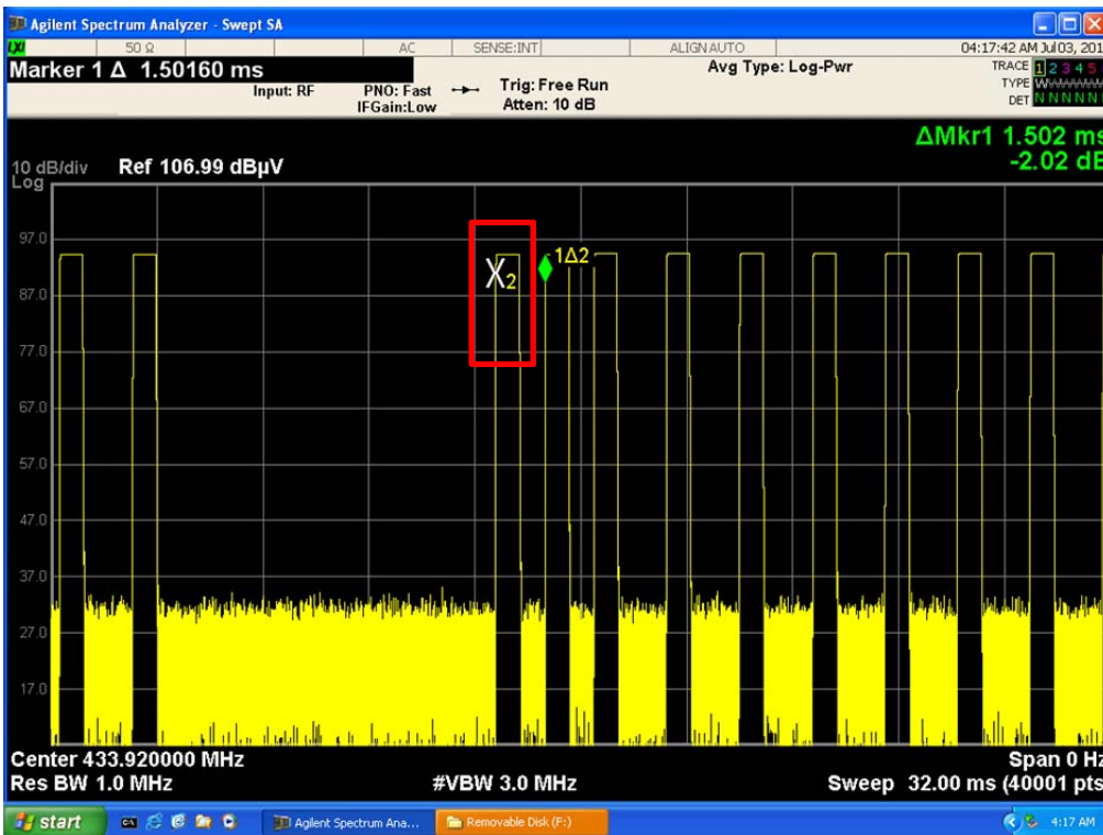
Period of Type 2 (Bit 0) : 1 502 μs
