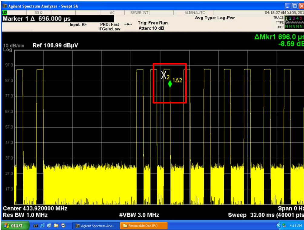
Duration Time of Type 3 (Bit 1) : 696.0 μs
