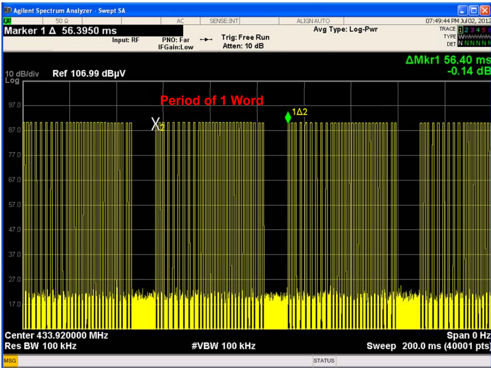
Period of 1 word : 56.40 ms
