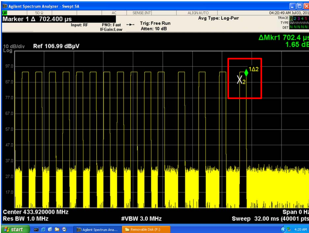
Duration Time of Type 4 (END) : 702.4 μs
