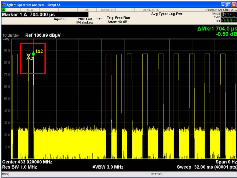
Duration Time of Type 1 (SYNC) : 704.0 μs
