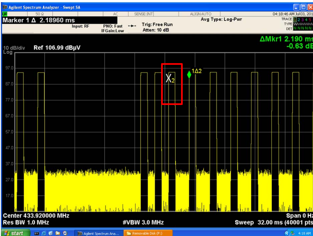
Period of Type 3 (Bit 1) : 2 190 μs
