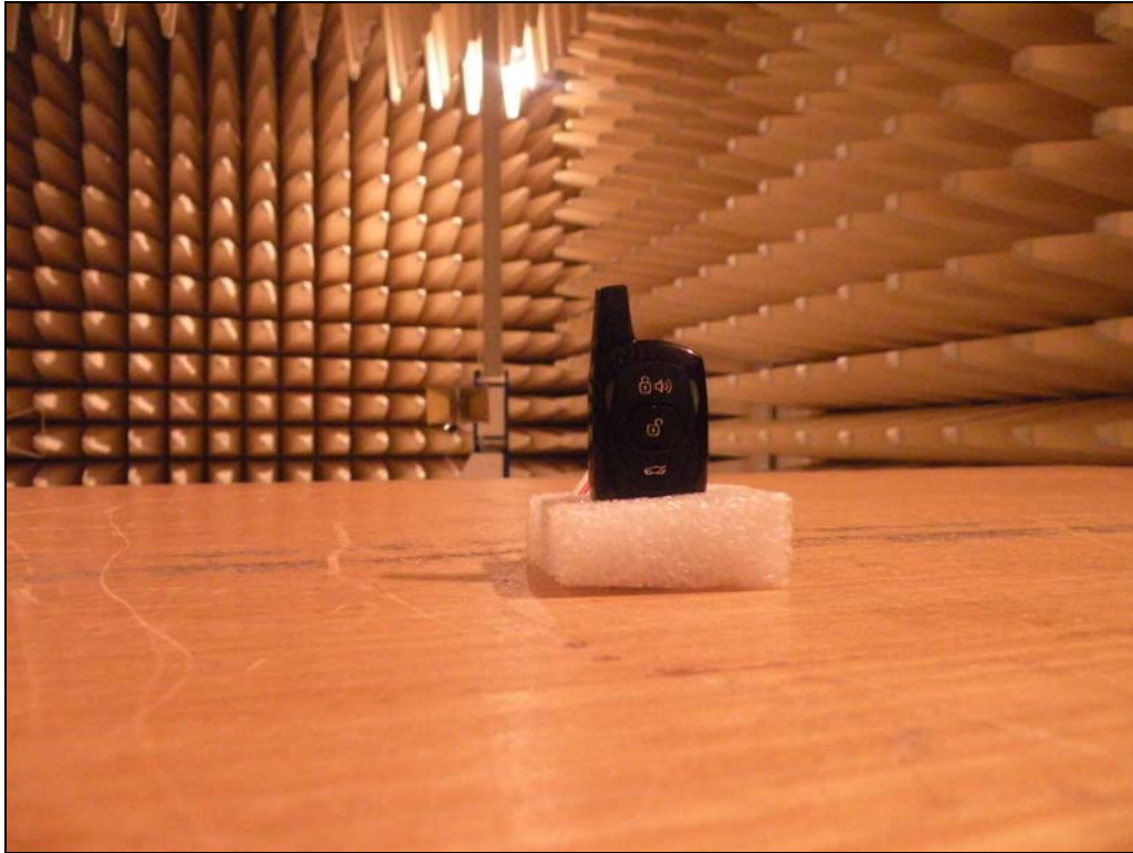
<Radiated Emission>
