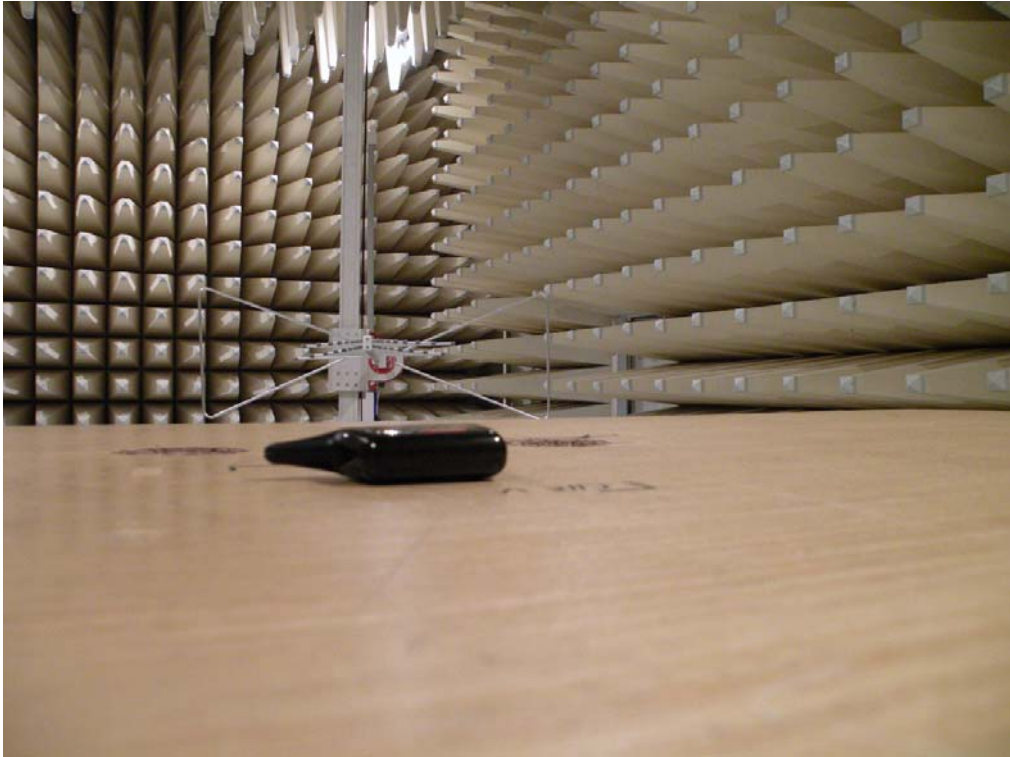
< Z-axis Radiated emission Test >
