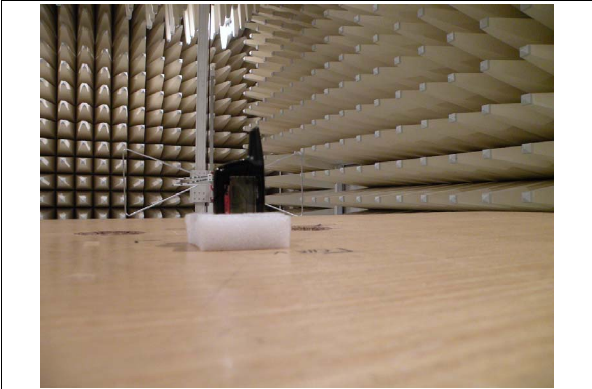
< X-axis Radiated emission Test >
