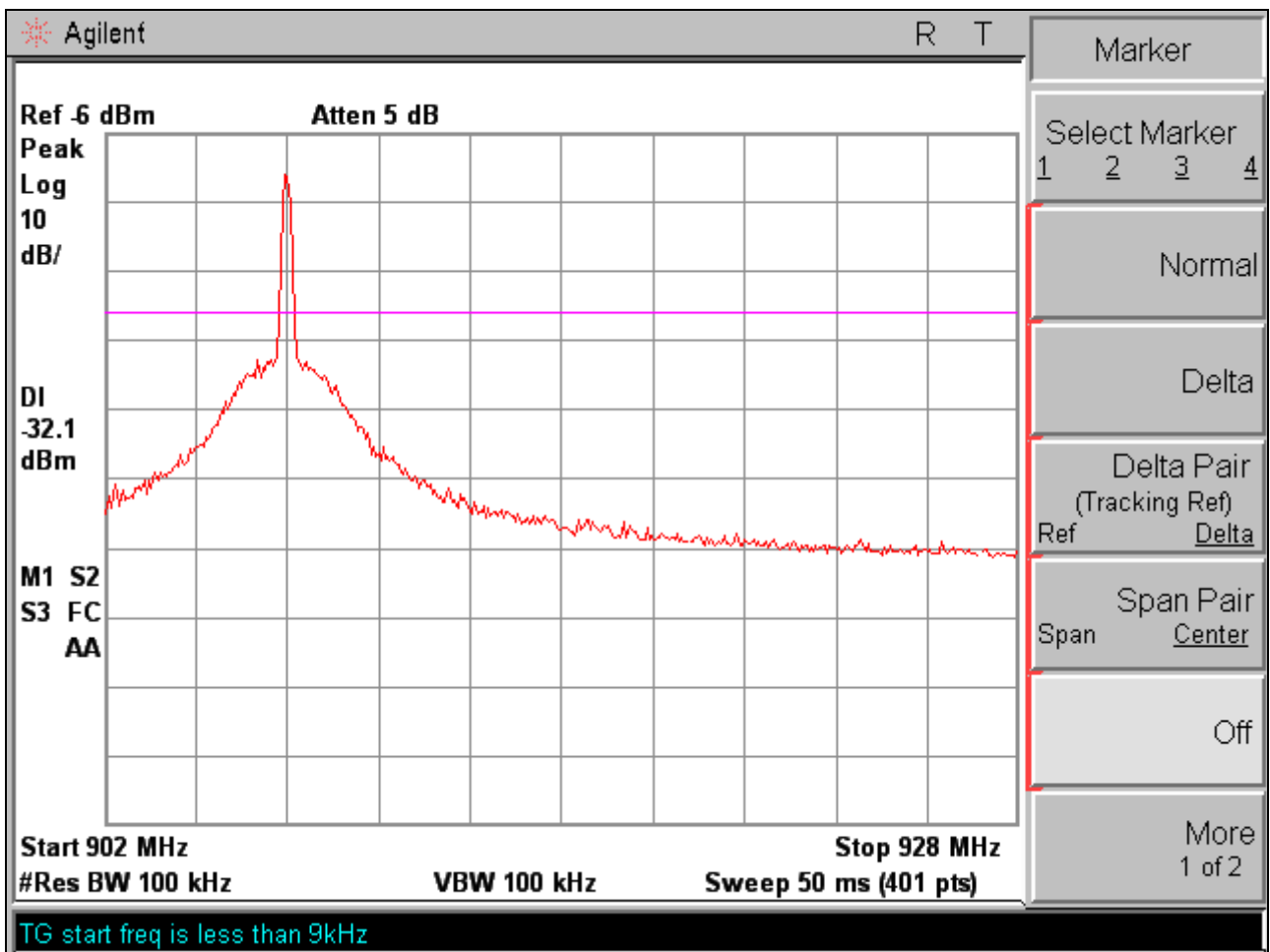
- Occupied Bandwidth plot -
