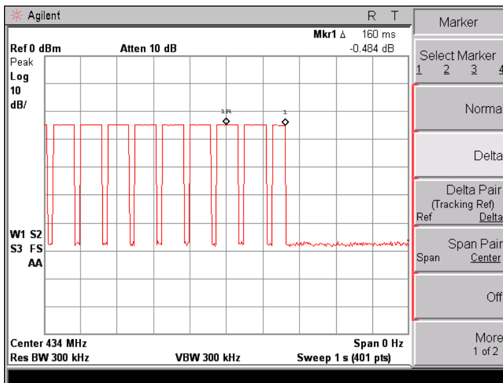
– Deactivation time –
