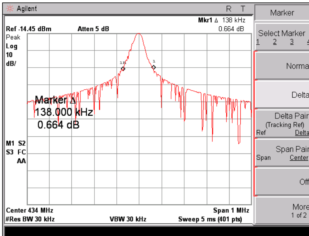
– 20 dB Bandwidth –
