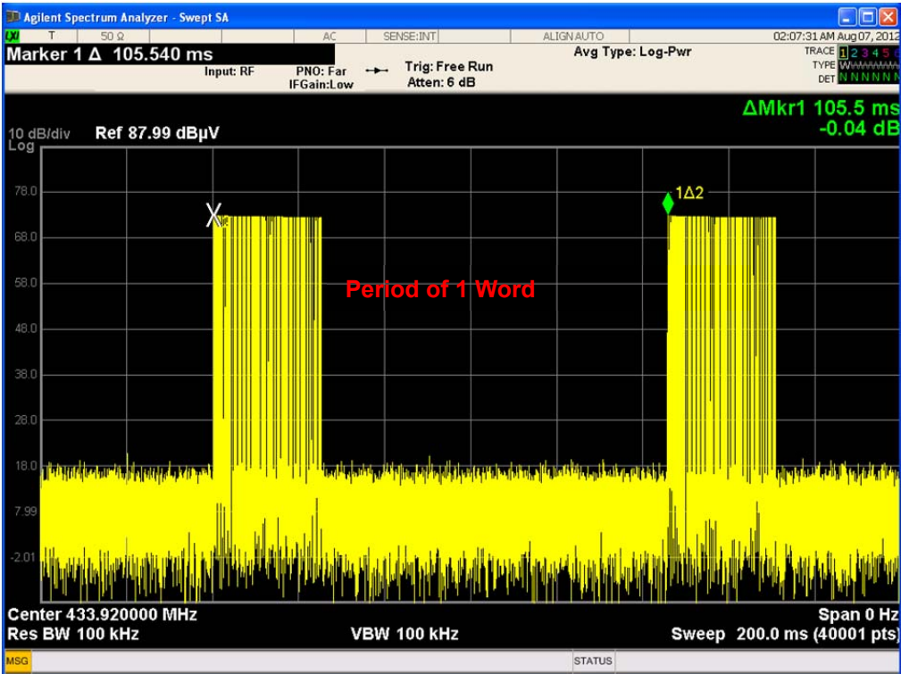
Period of 1 word : 105.5 ms
