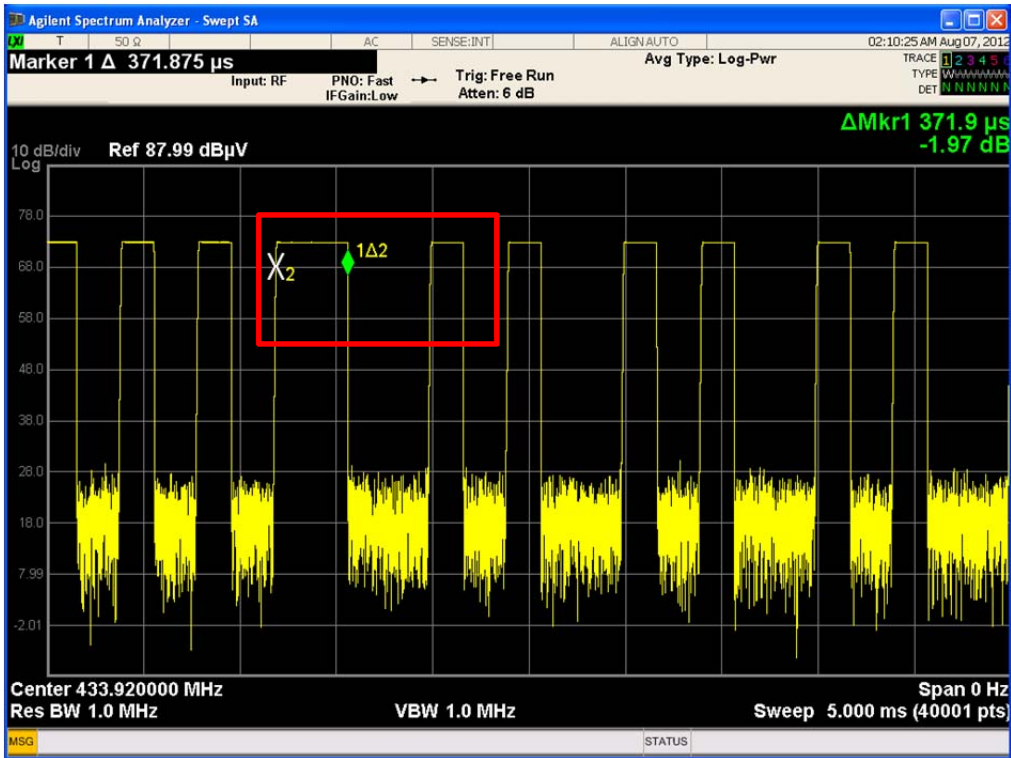
Duration Time of Type 1 (1 st Data) : 371.9 μs
