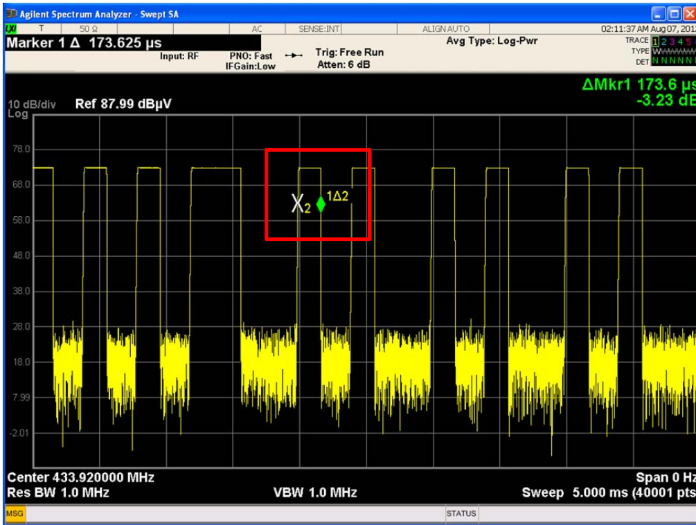
Duration Time of Type 1 (2 nd Data) : 173.6 μs
