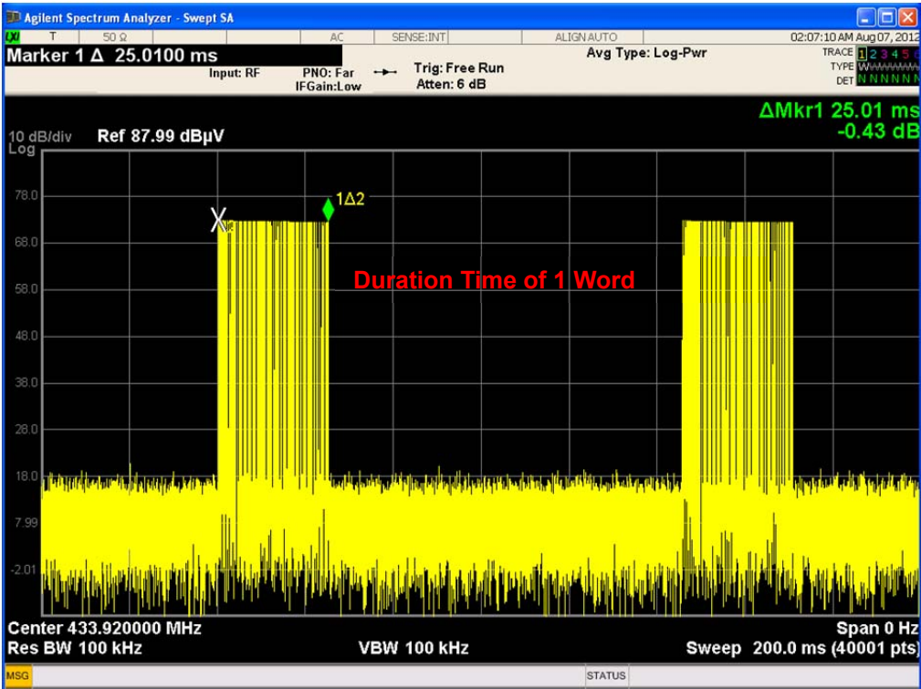
Duration Time of 1 word : 25.01 ms
