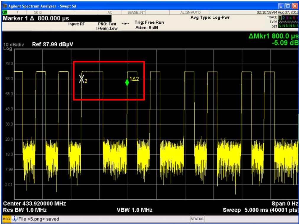
Period of Type 1 (1 st Data) : 800.0 μs
