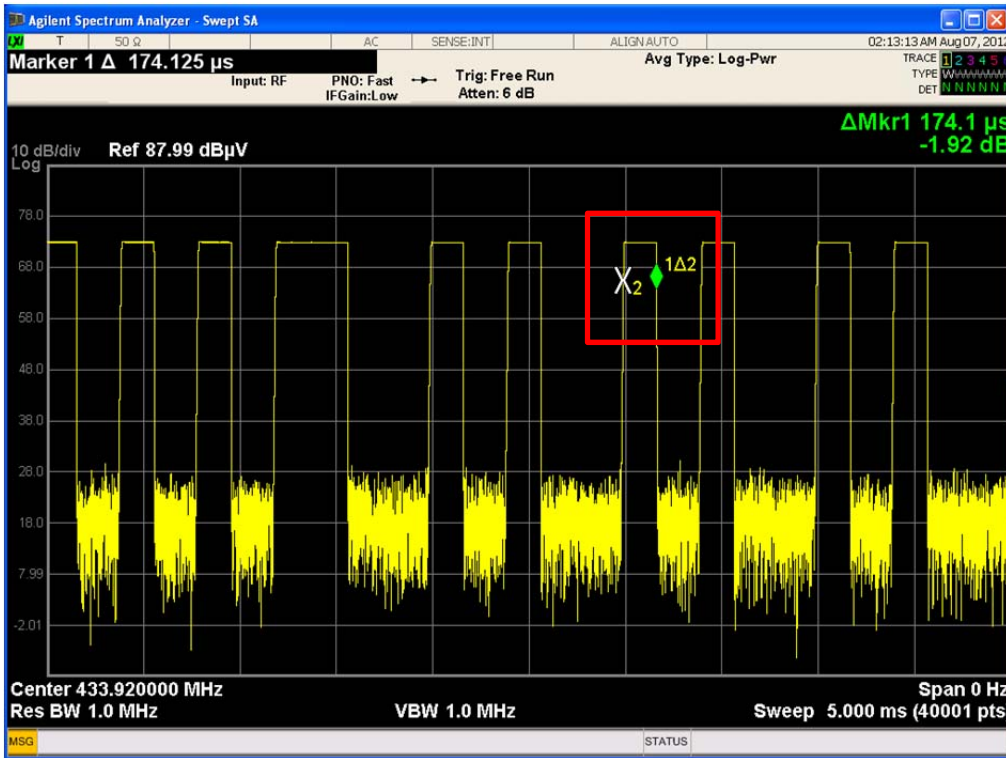
Duration Time of Type 2 (Bit 0) : 174.1 μs
