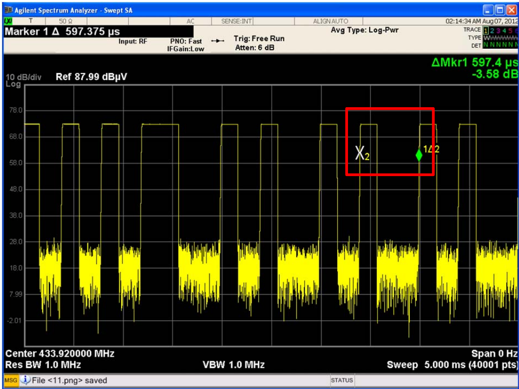
Period of Type 3 (Bit 1) : 597.4 μs
