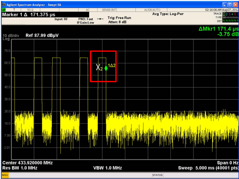
Duration Time of Type 4 (Bit 0) : 171.4 μs
